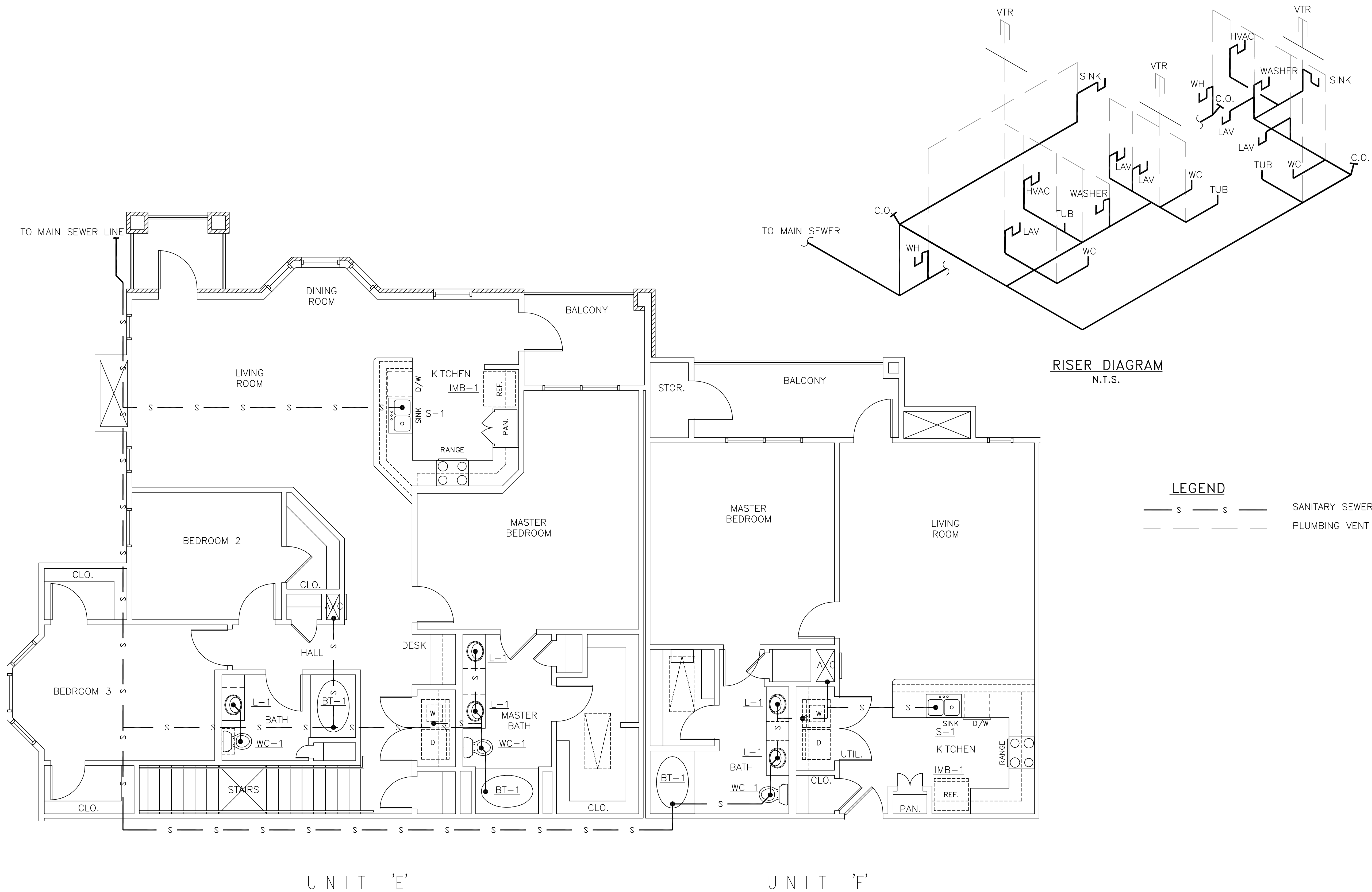
UNITS E & F PLUMBING PLAN SCALE: 1/4" = 1'-0"
