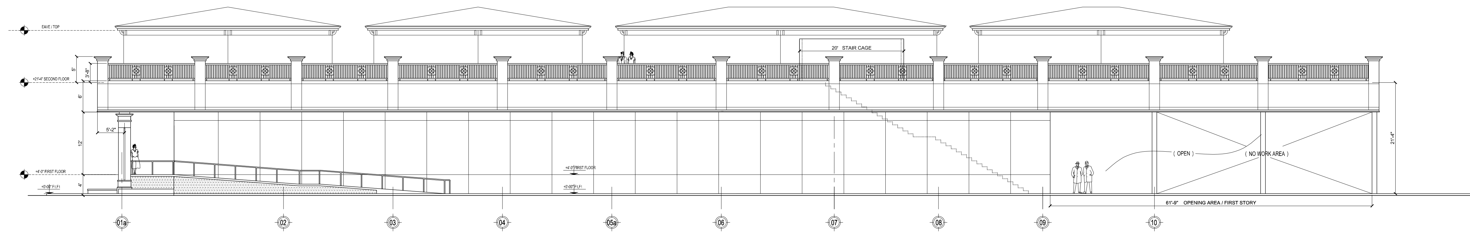
SIDE ELEVATION - ST SALCEDO ST VIEW SCALE : 1" = 10'-0" -SEE : MATERIAL FOR EXT. BLDG AT " FRONT ELEVATION "
