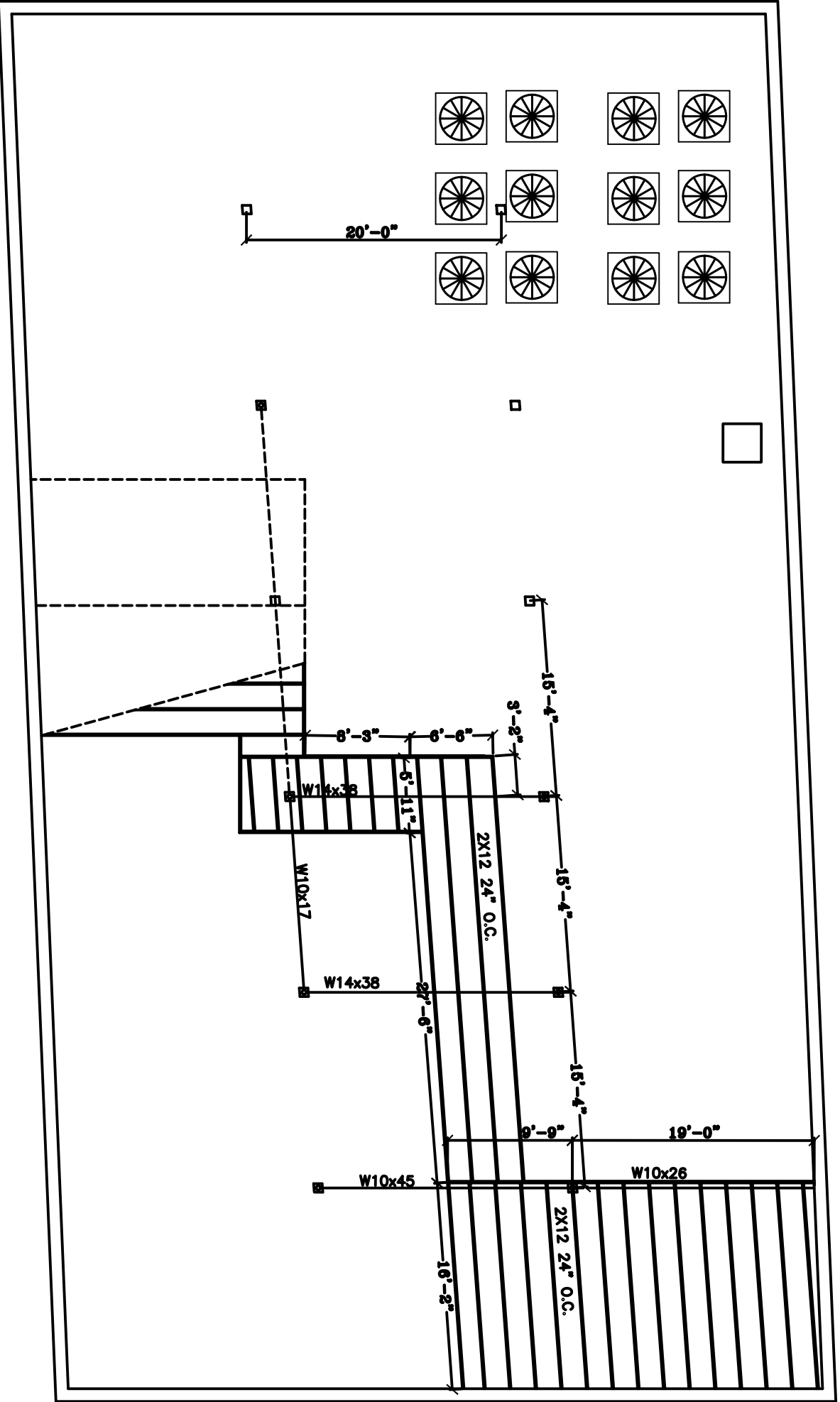
FRAMING PLAN SCALE: 3/32" = 1'-0"
