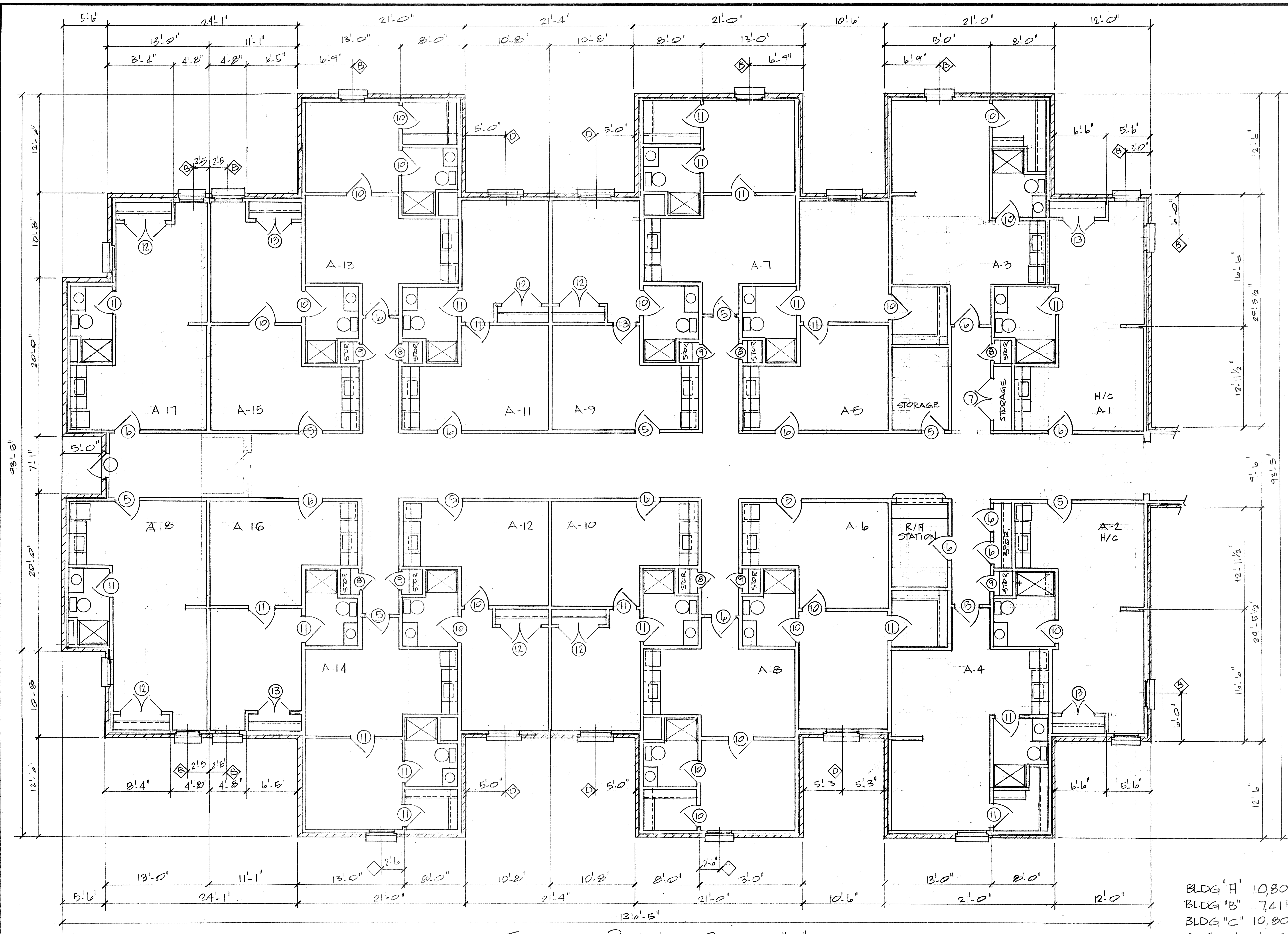
FLOOR PLAN BLDG "A" SCALE 3/16" = 1'-0"
