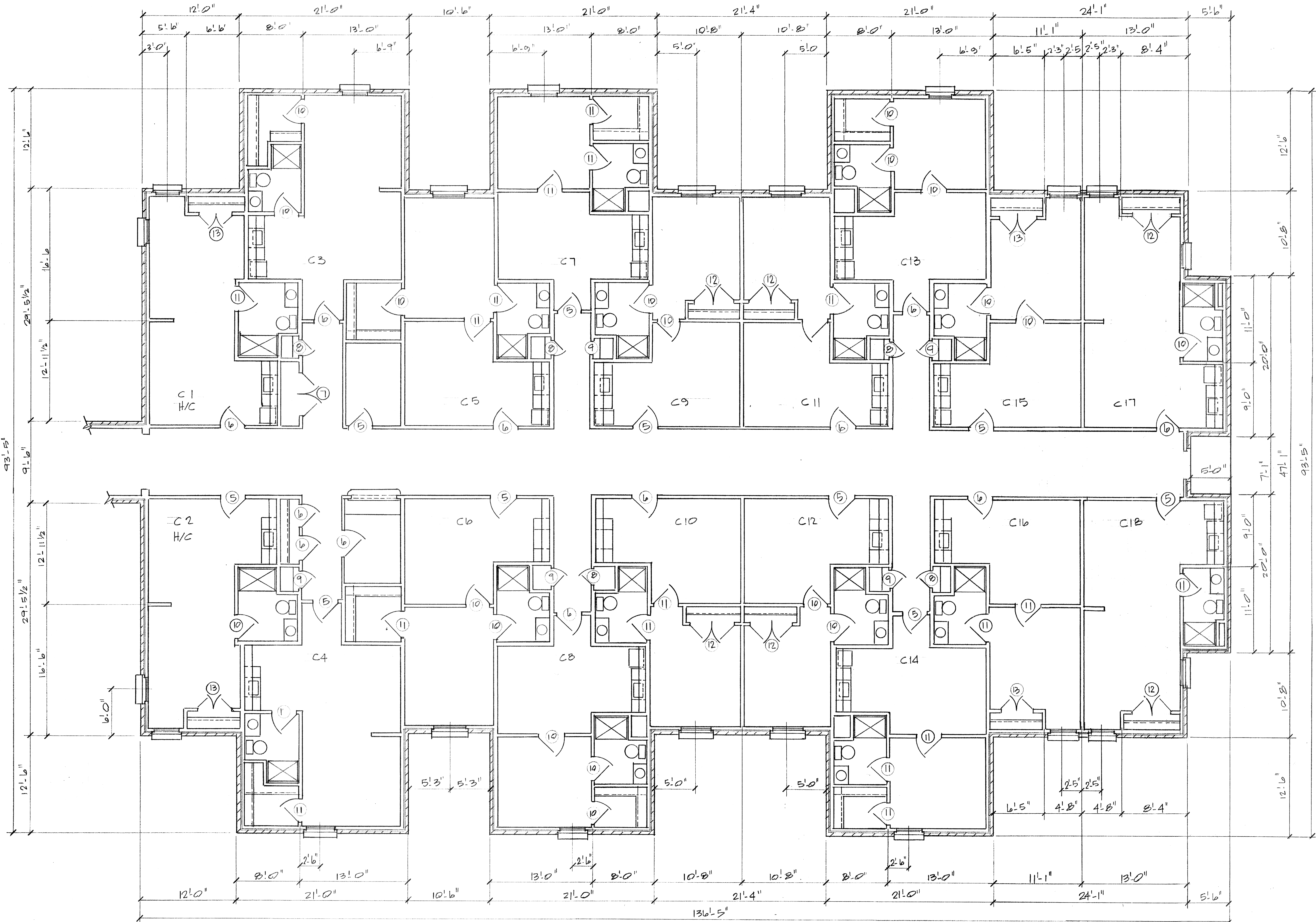
FLOOR PLAN BLDG. "C" SCALE 3/16 = 1'-0"
