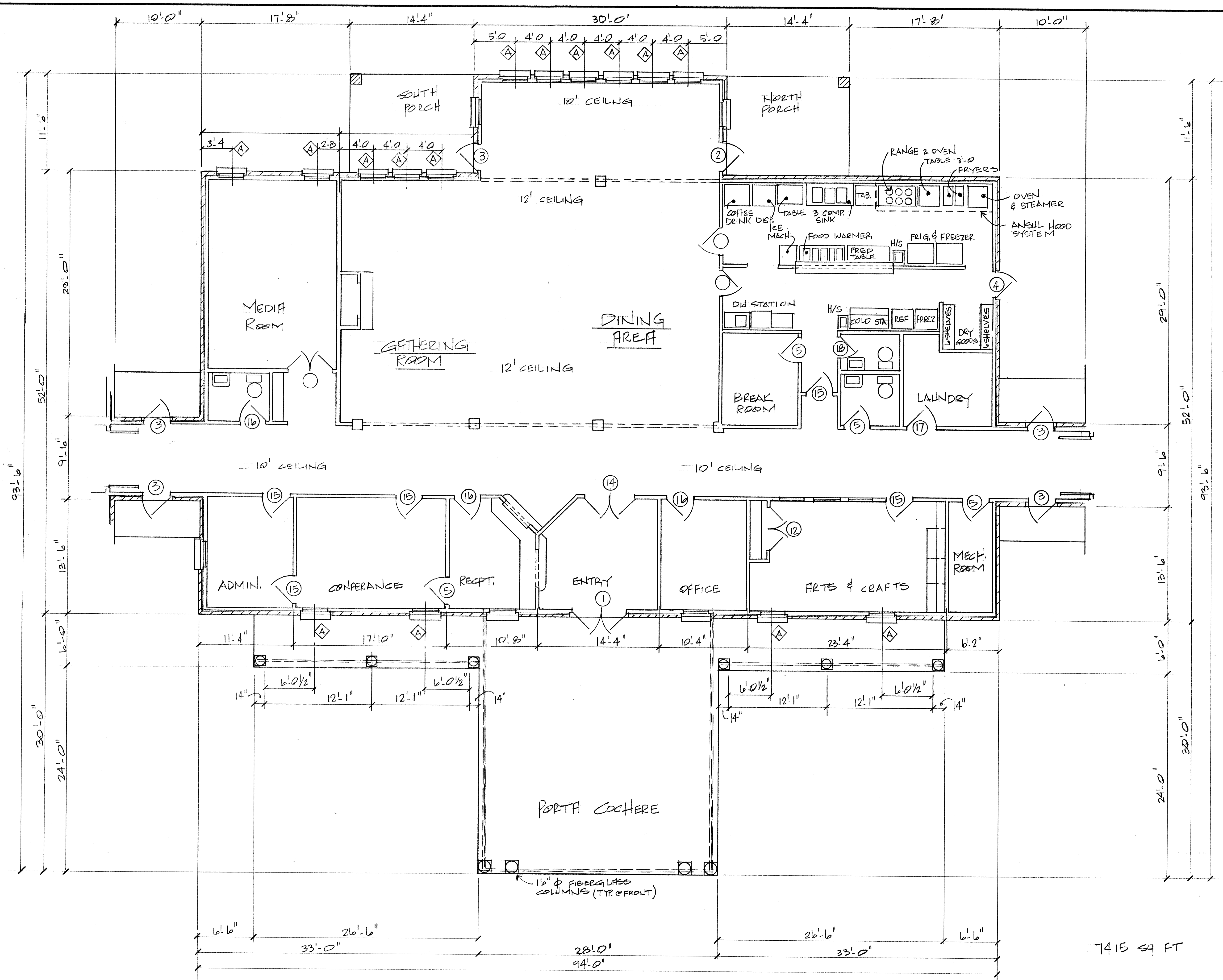
BUILDING "B" FLOOR PLAN SCALE 3/16" = 1'-0"
