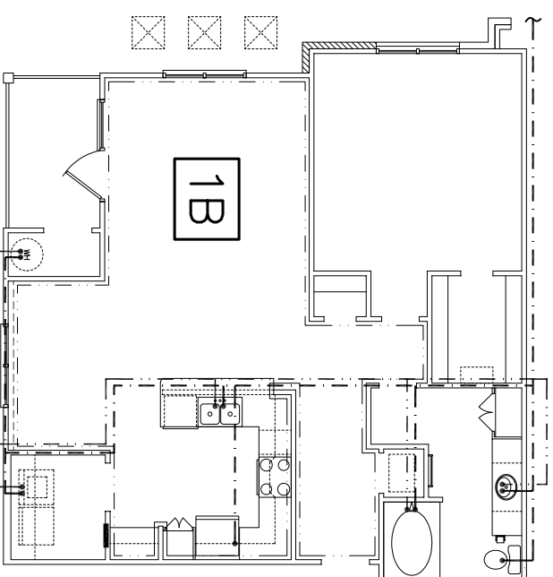
UNIT 1B WATER PLUMBING PLAN SCALE 1/4" = 1'-0"
