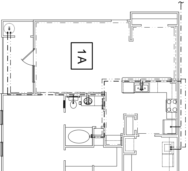
UNIT 1A WATER PLUMBING PLAN SCALE 1/4" = 1'-0"
