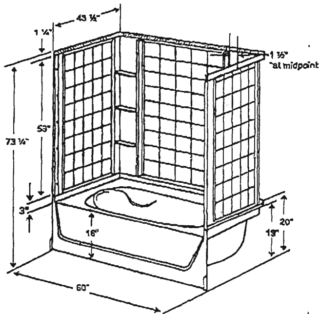
Fixture Dimensions
