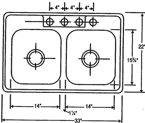
Bowl Depth is 6" Model K-23322-4 Illustrated
