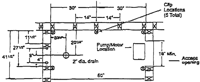
Framing Dimensions
