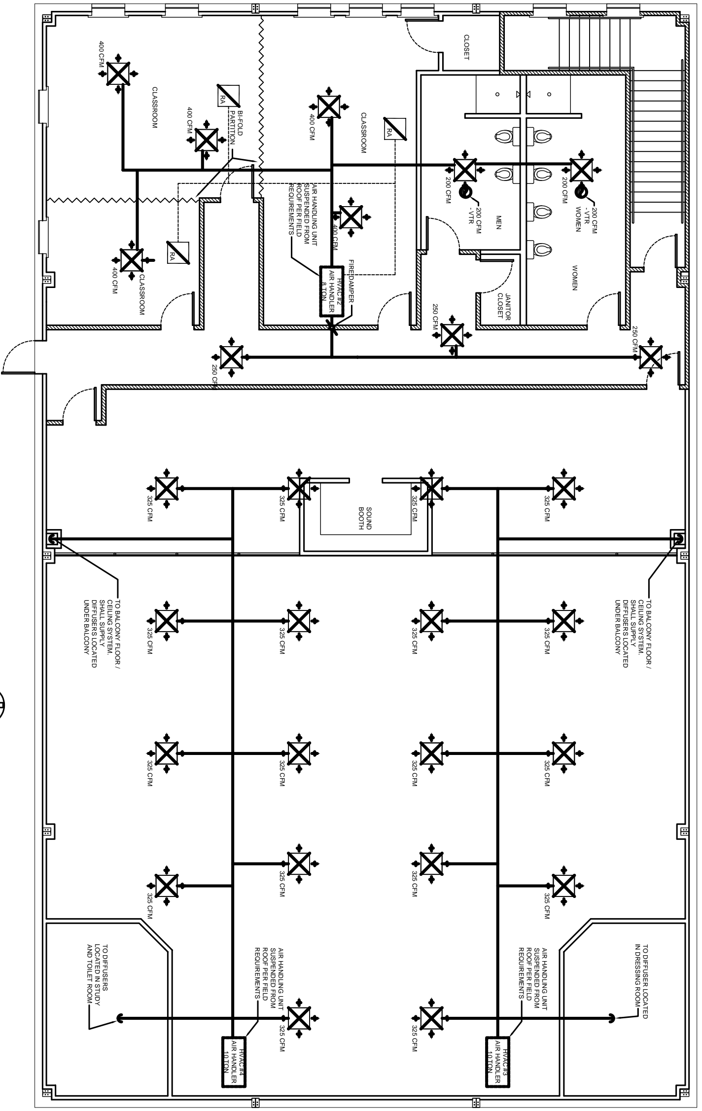
2nd FLOOR MECHANICAL PLAN SCALE: 1/4"=1'-0"
