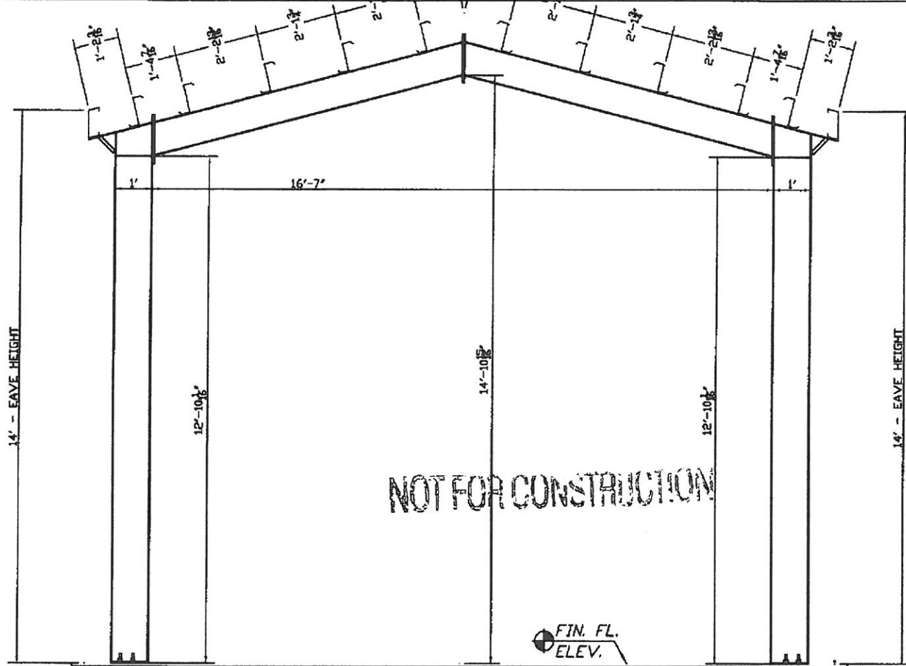
CROSS SECTION AT FRAME LINE '1' - (B) b
