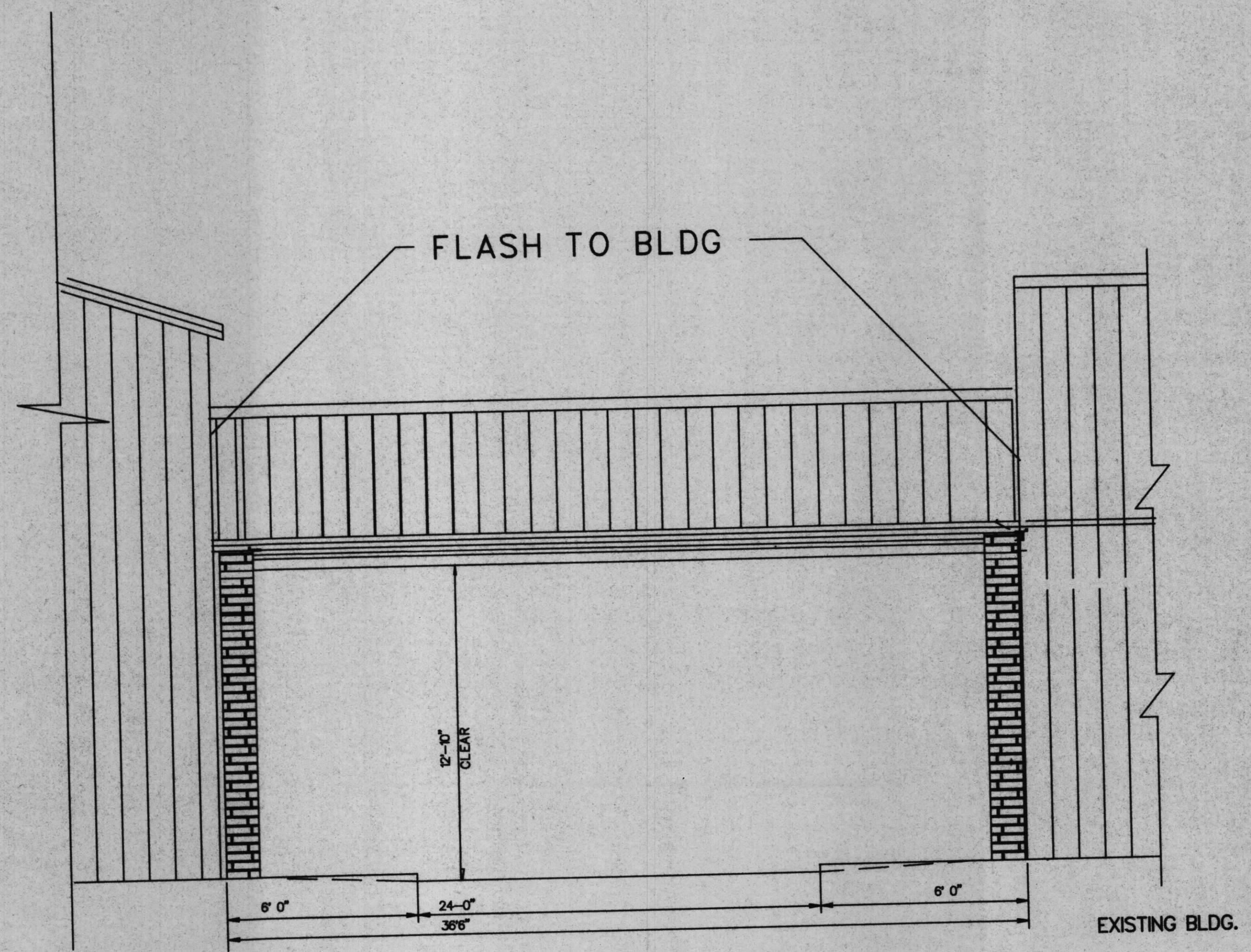
SIDE ELEVATION
