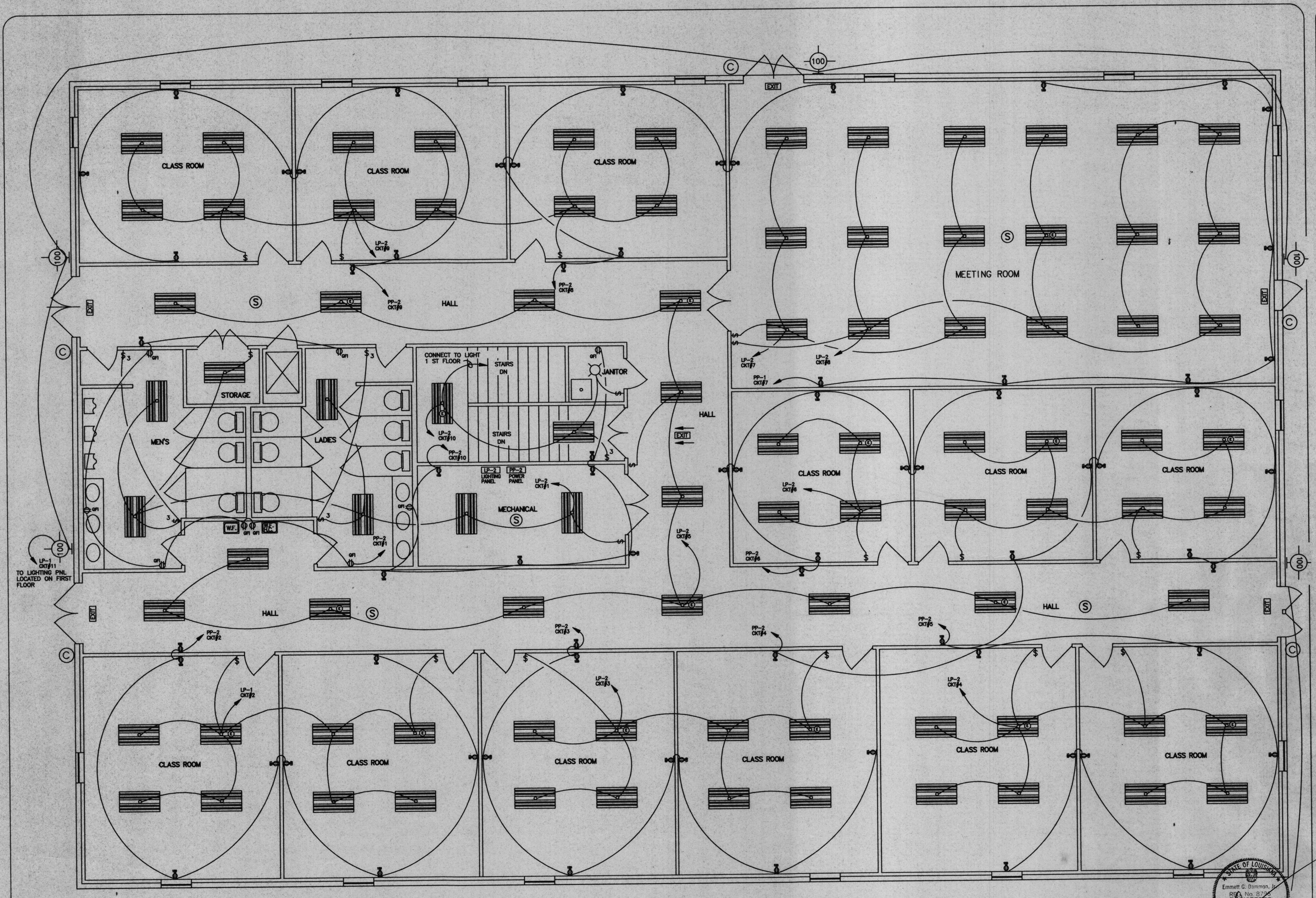
ELECTRICAL PLAN -2nd FLOOR SCALE: 1/4"=1'-0"
