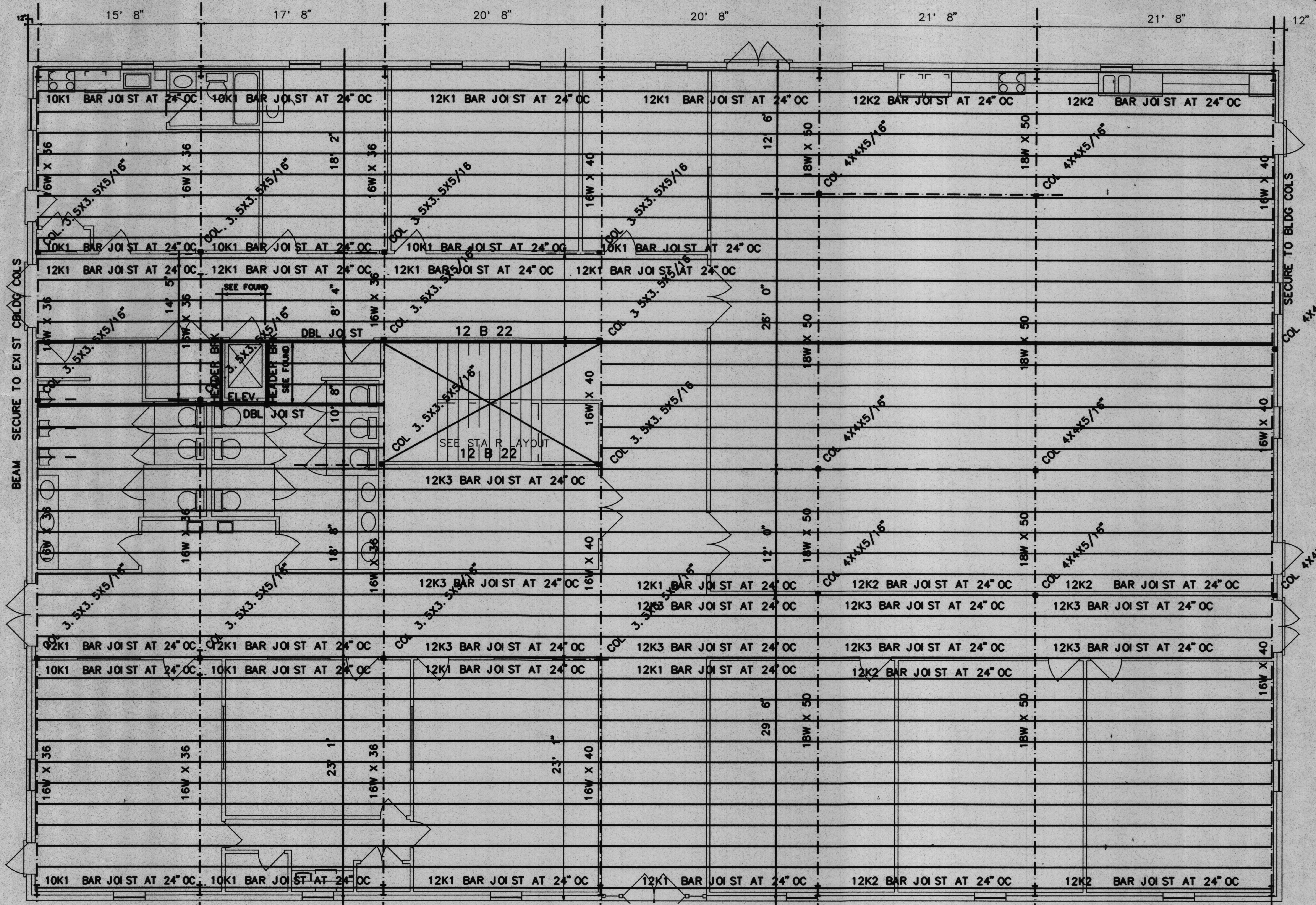
PRELIMINARY 1ST FLOOR FRAMING PLAN
