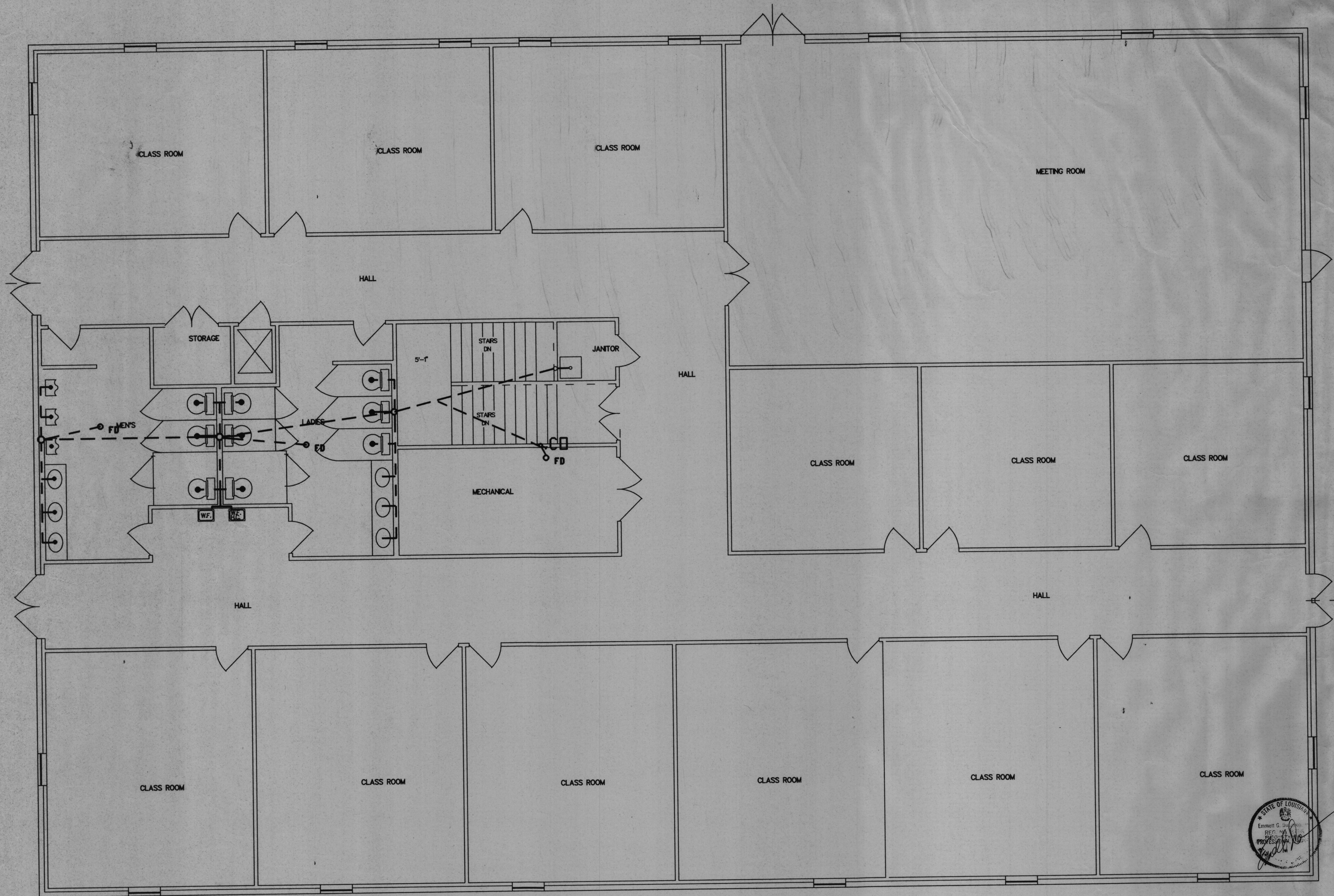
PLUMBING PLAN-2nd FLOOR
