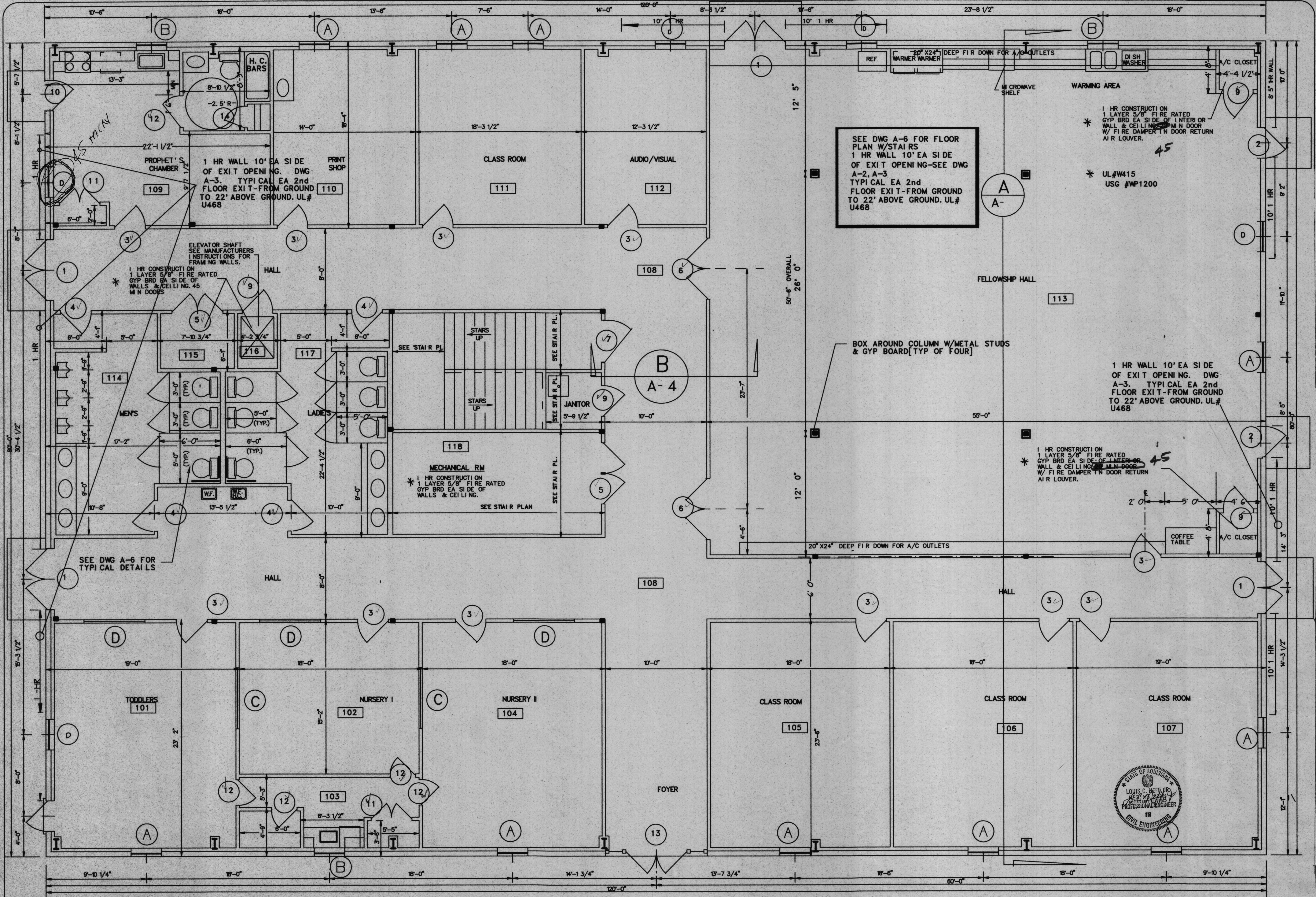
1st FLOOR PLAN SCALE 1/4"=1'-0"
