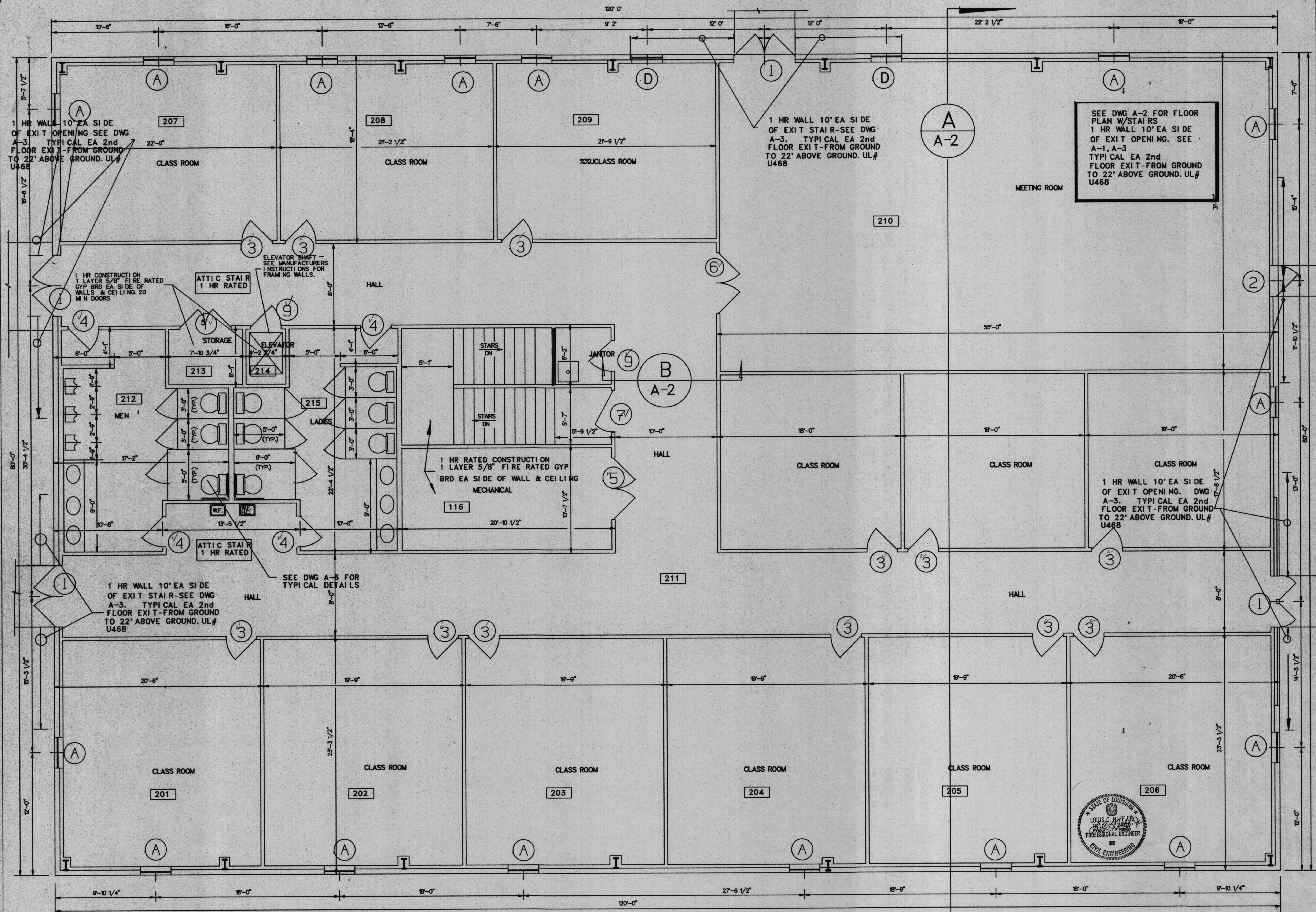
2nd FLOOR PLAN SCALE 1/4"=1'-0"
