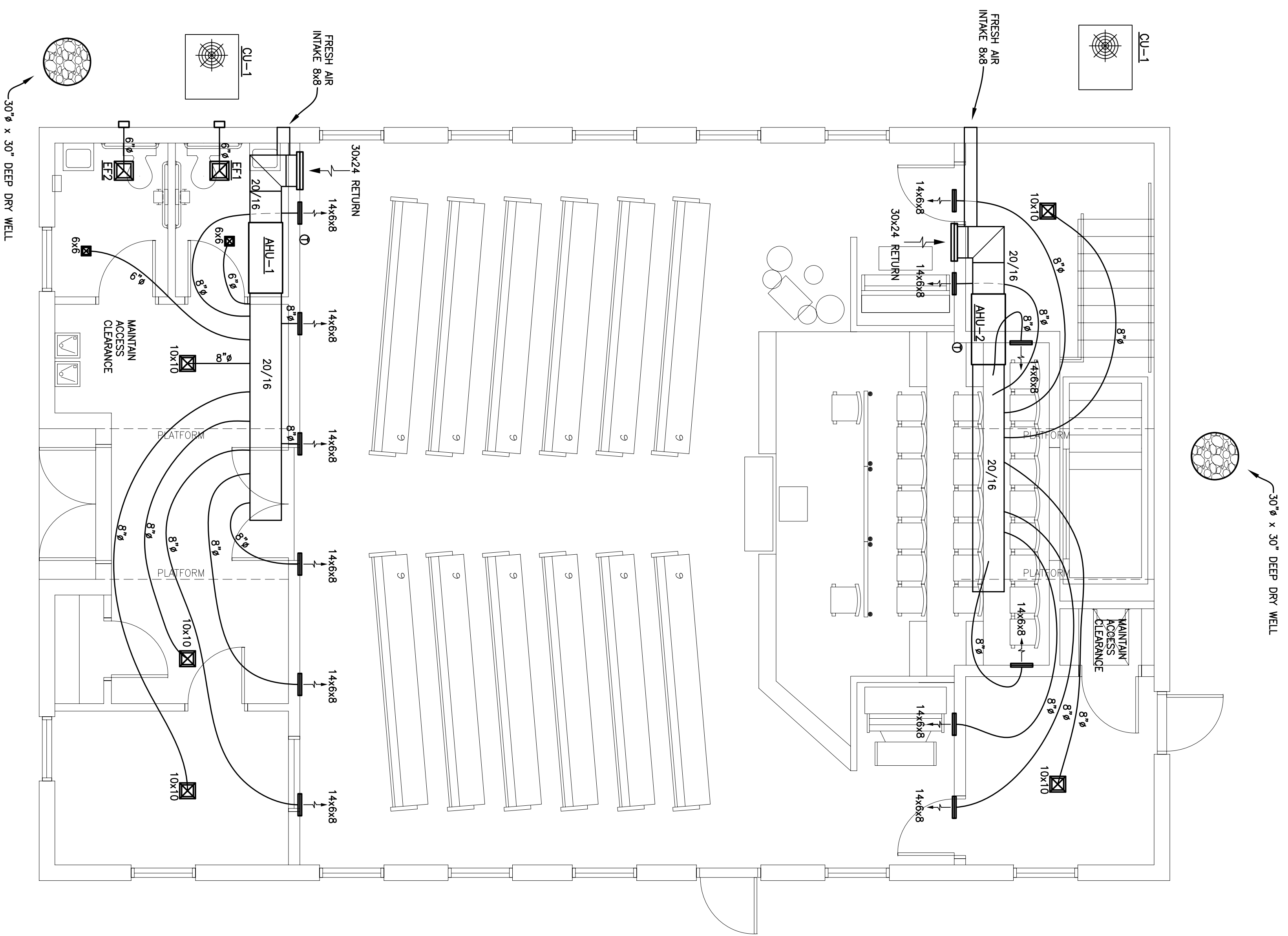
1 MECHANICAL PLAN M2.1 SCALE: 1/4" = 1'-0"
