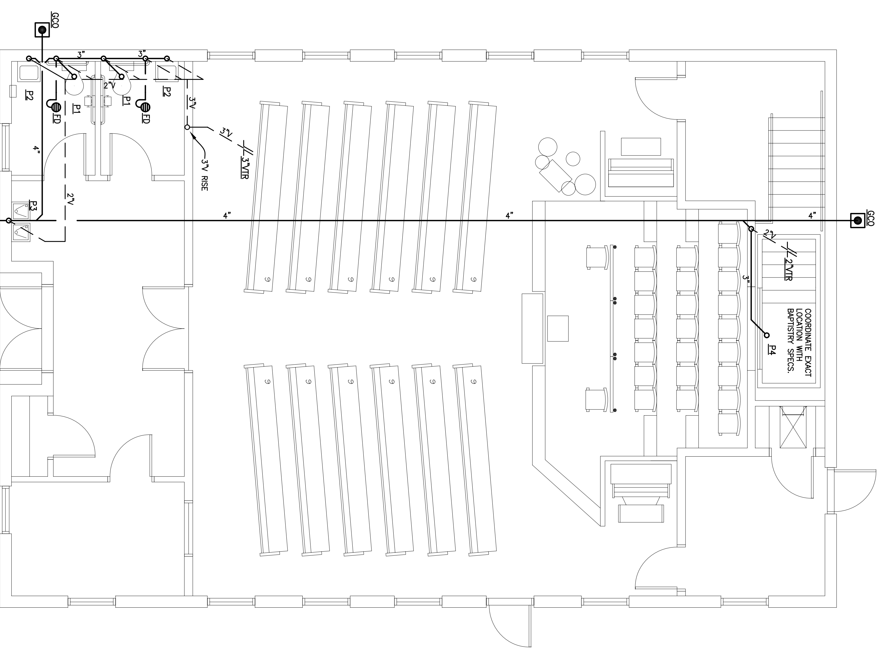
2 SANITARY AND VENT PIPING PLAN P2.1 SCALE: 1/4" = 1'-0"
