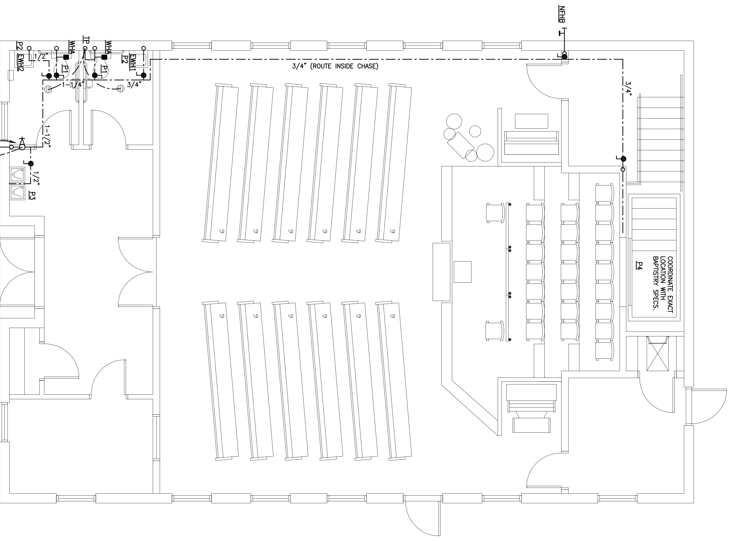
1 POTABLE WATER PIPING PLAN P2.1 SCALE: 1/4" = 1'-0"
