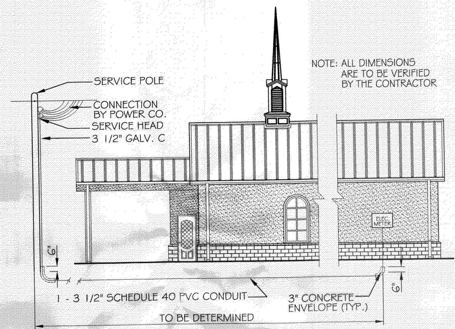
ELECTRICAL SERVICE DETAIL NTS
