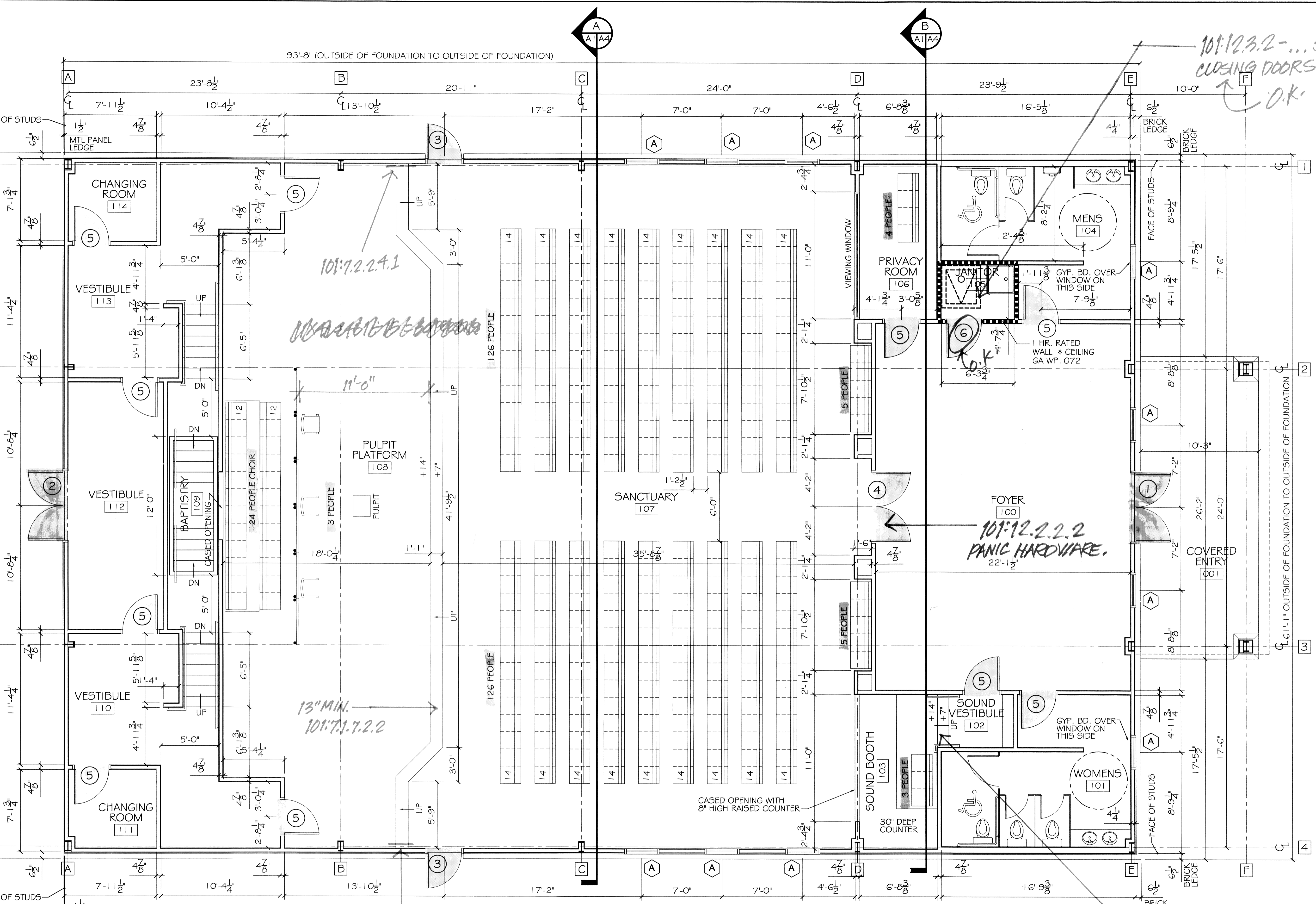
FLOOR PLAN SCALE: 1/4" = 1'
