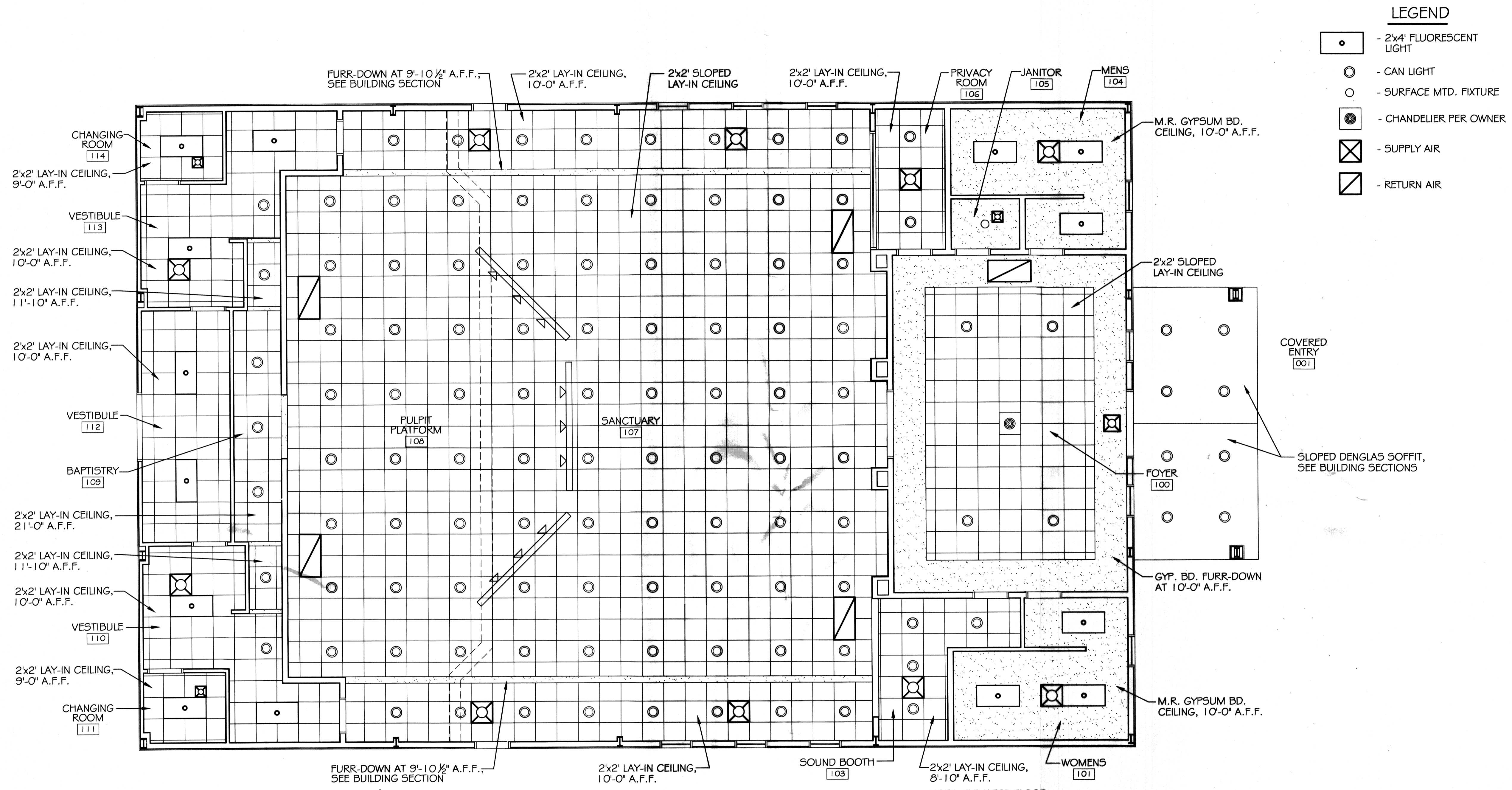
REFLECTED CEILING PLAN SCALE: 3/16"=1'
