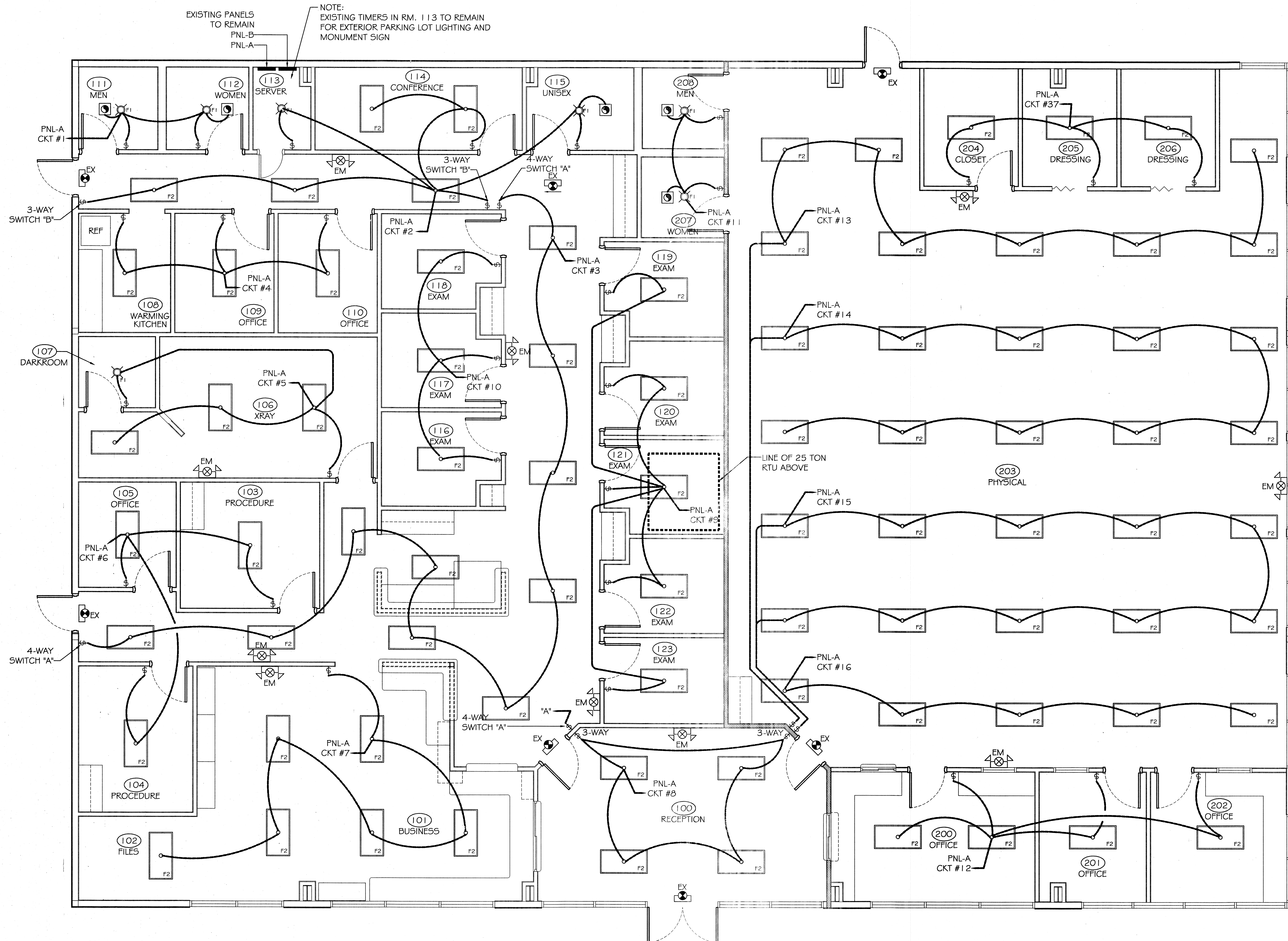
LIGHTING PLAN SCALE: 1/4" = 1'-0"
