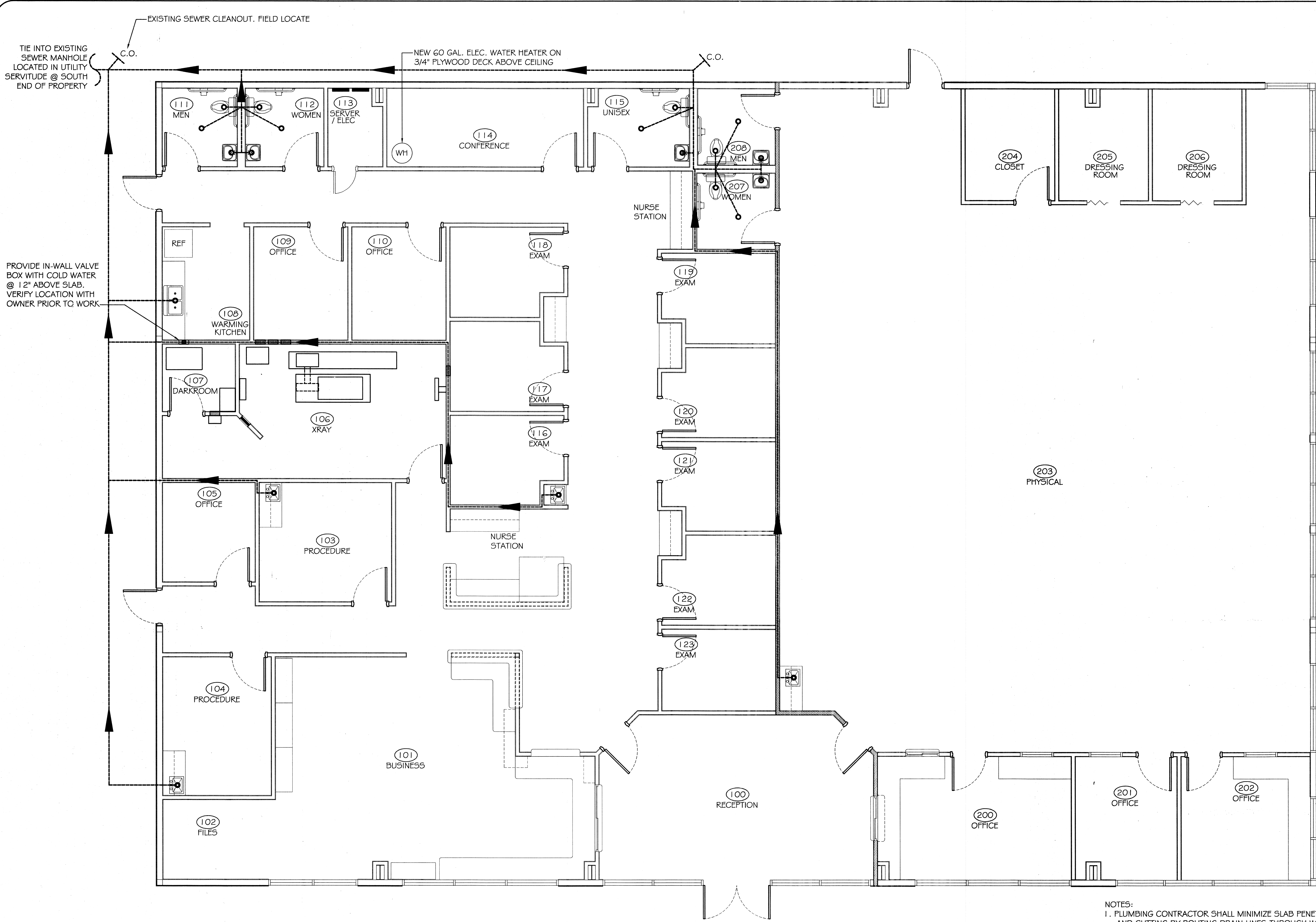
PLUMBING PLAN SCALE: 1/4" = 1'-0"
