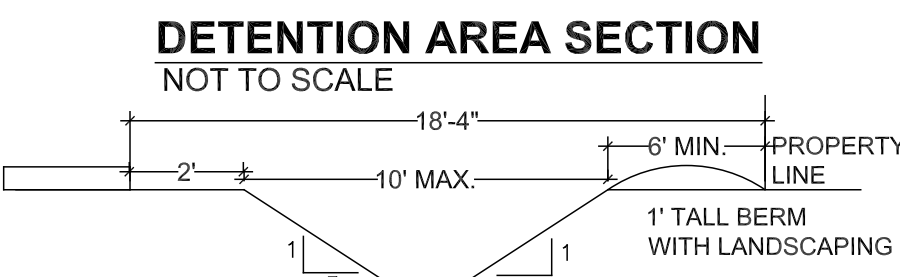
SOUTH SWALE SECTION NOT TO SCALE
