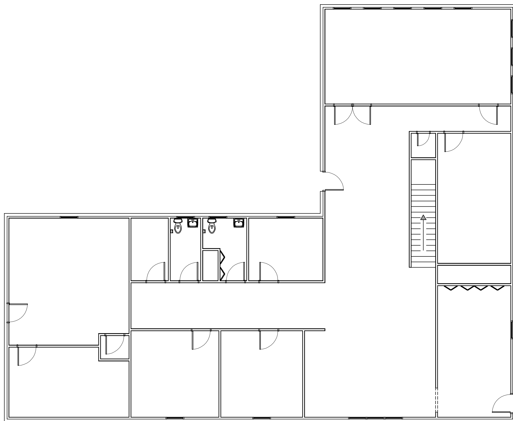
2 EXISTING FLOOR PLAN LEVEL ONE SCALE: 1/8"=1'-0"
