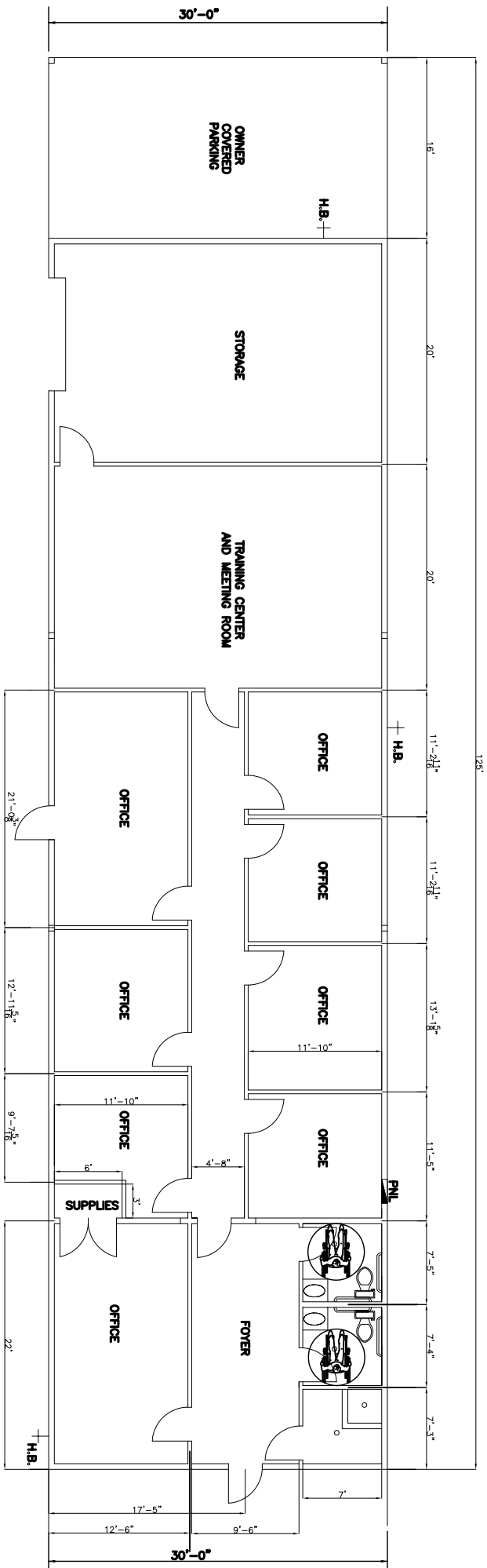
FLOOR PLAN
