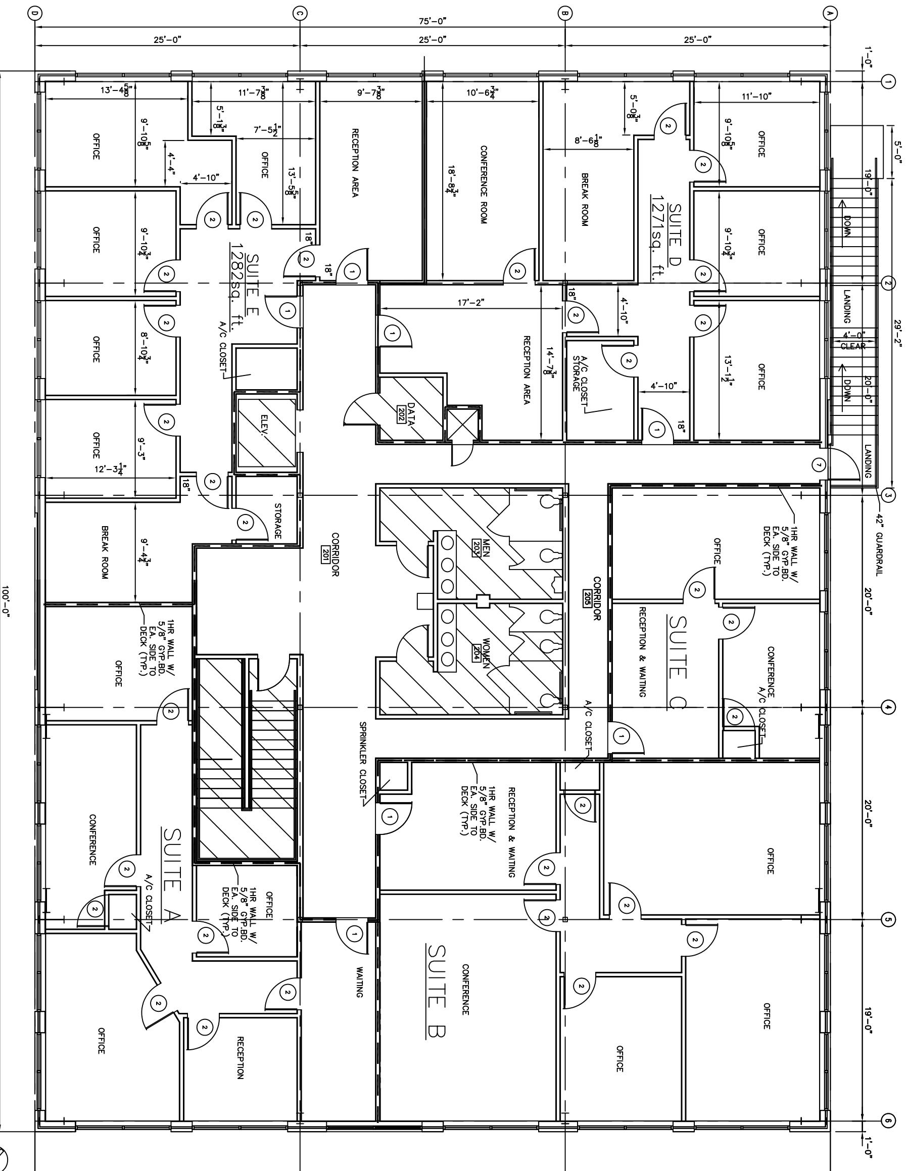
1 FLOOR PLAN-SECOND FLOOR A-1 3/16"=1'-0"
