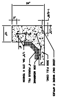
1 SECTION (EXTERIOR BEAMS) 1'-11 1/2\"/>
