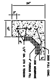
2 SECTION (EXTERIOR BEAMS) 1'-11 1/2\"/>
