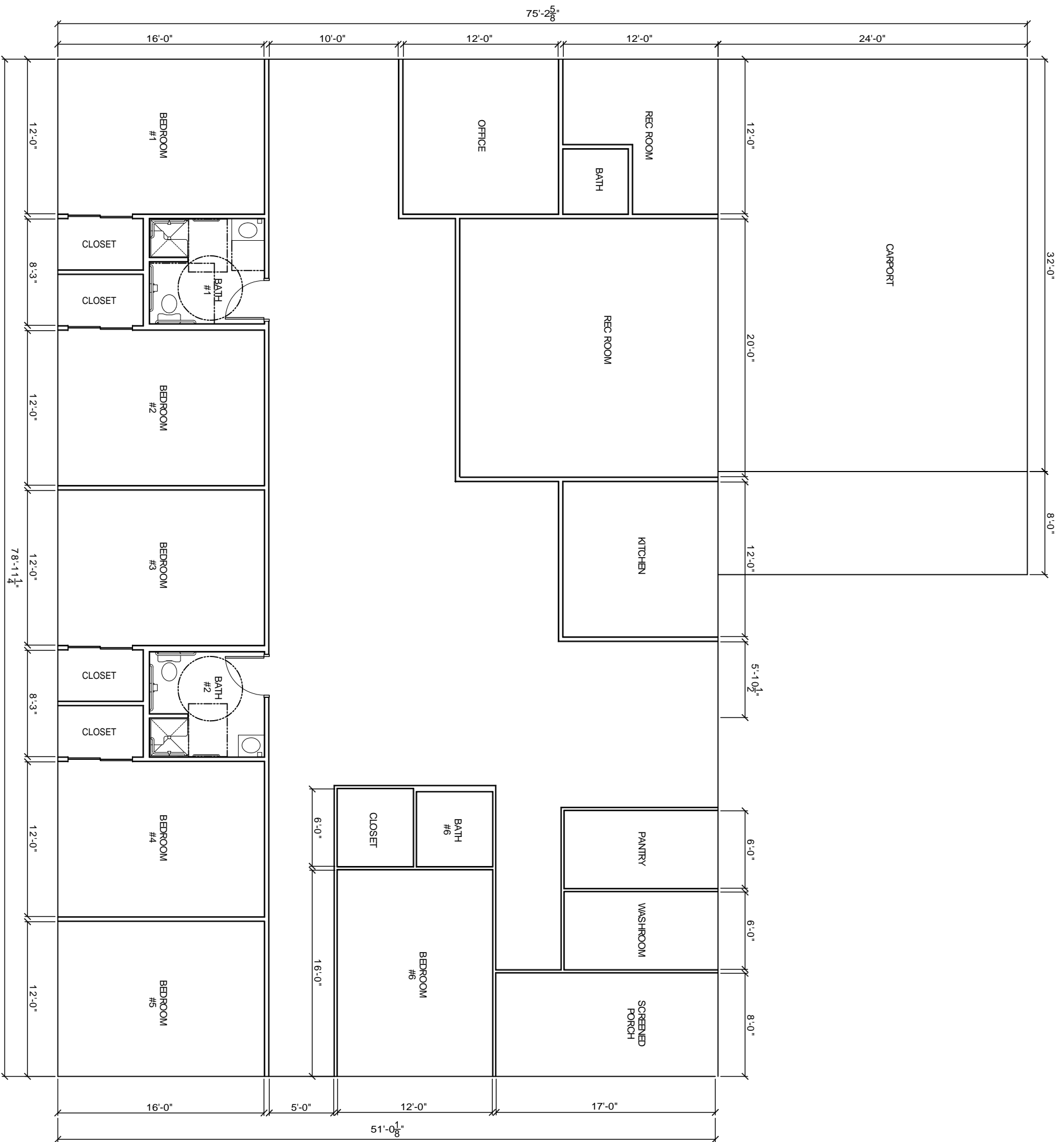
PRELIM. FLOOR PLAN #1 SCALE: 1/4" = 1'
