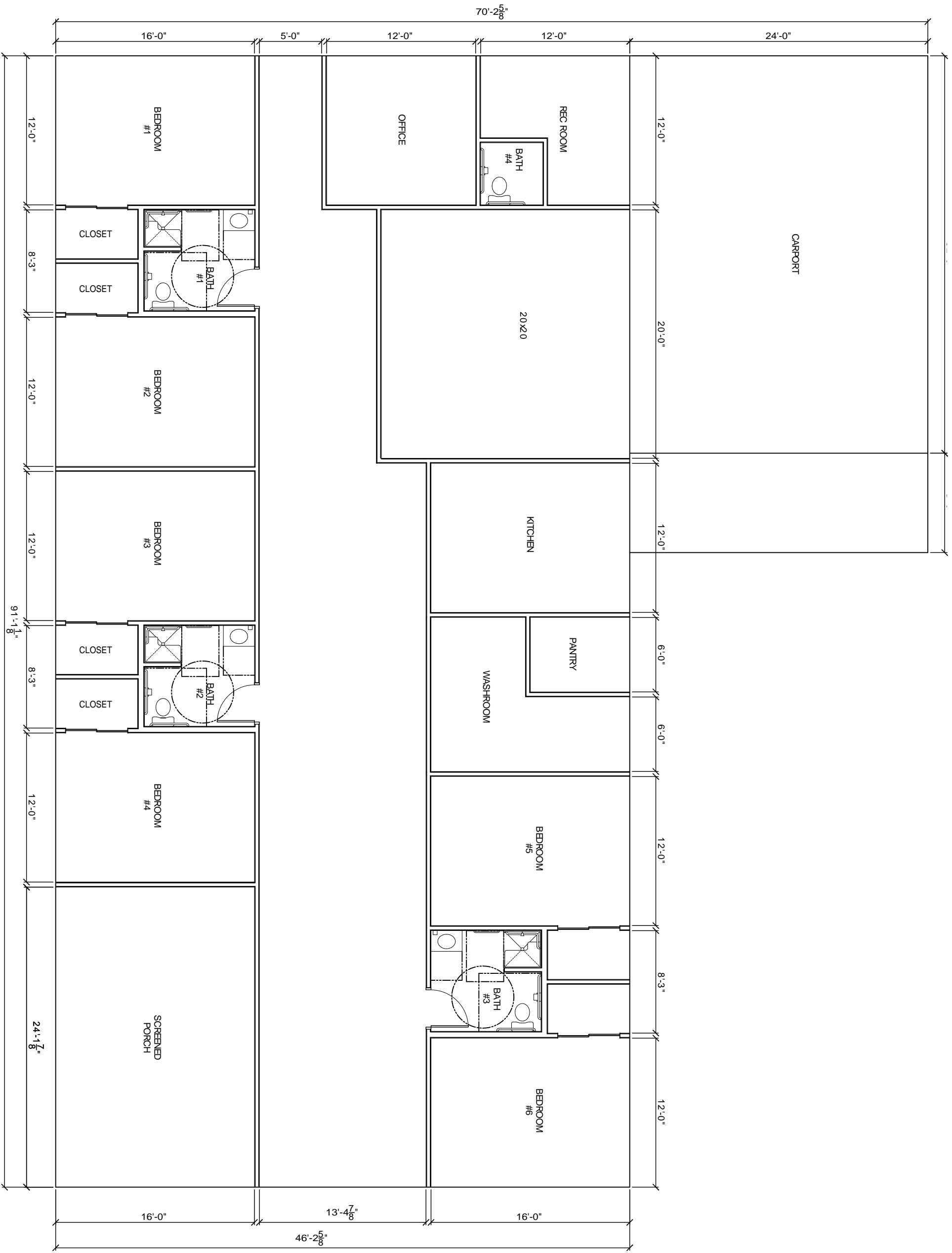
PRELIM. FLOOR PLAN #3 SCALE 1/4" = 1'
