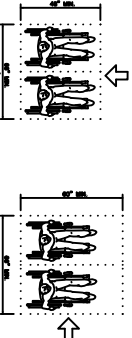
SPACE REQUIREMENTS FOR WHEELCHAIR SEATING SPACES IN SERIES
