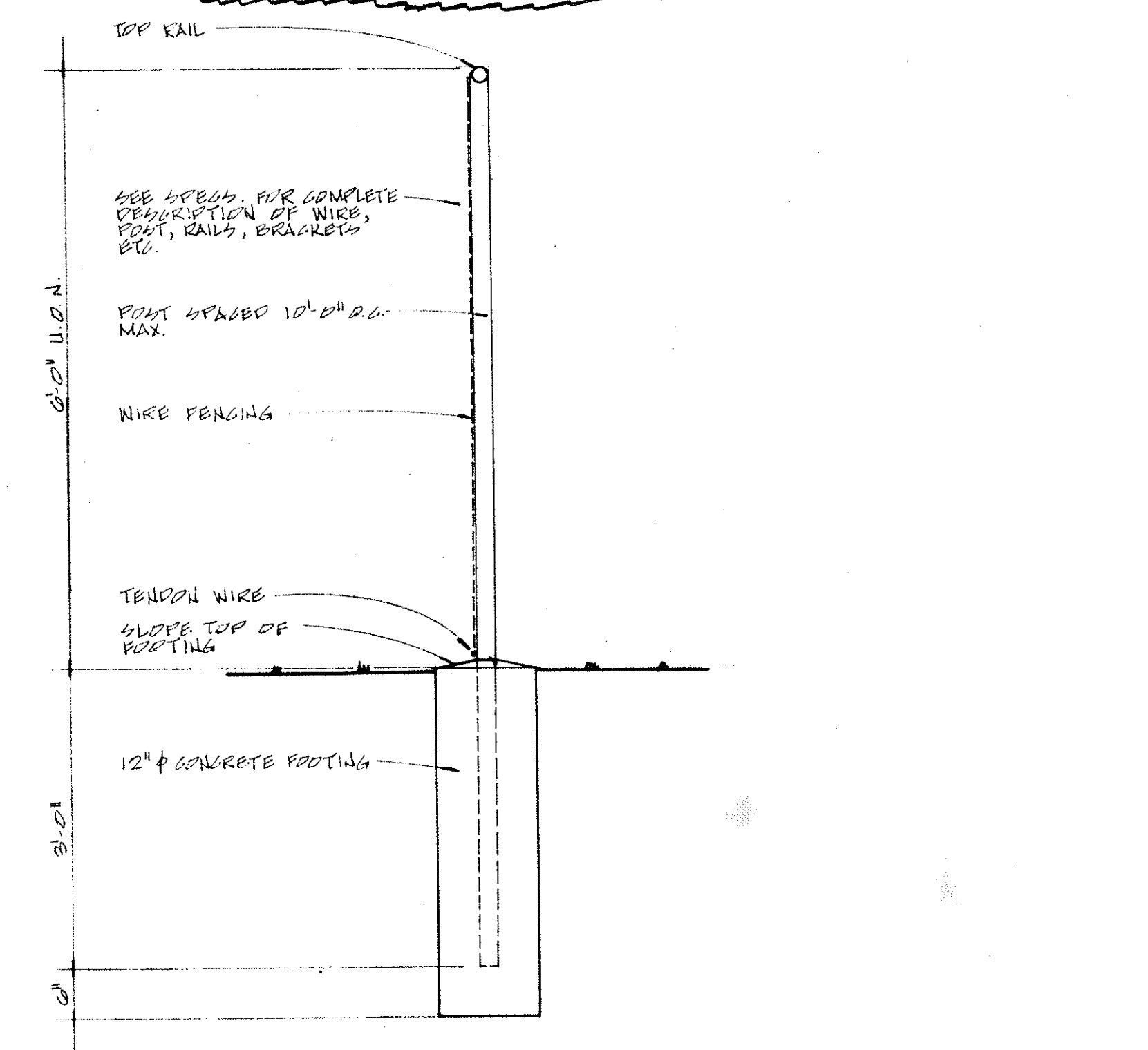
3 CHAINLINK FENCE DETAIL
