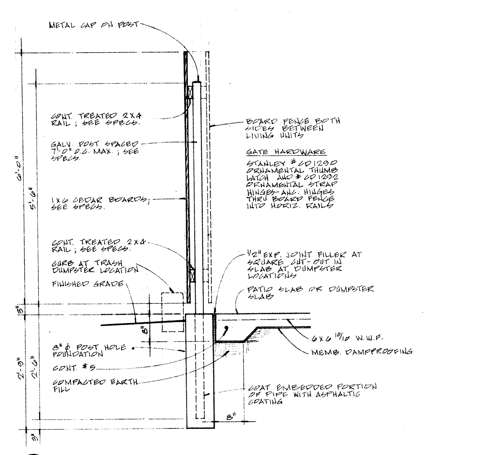
2 BOARD FENCE DETAIL - AT TRASH ENCLOSURE AND AT PATIO ENCLOSURE
