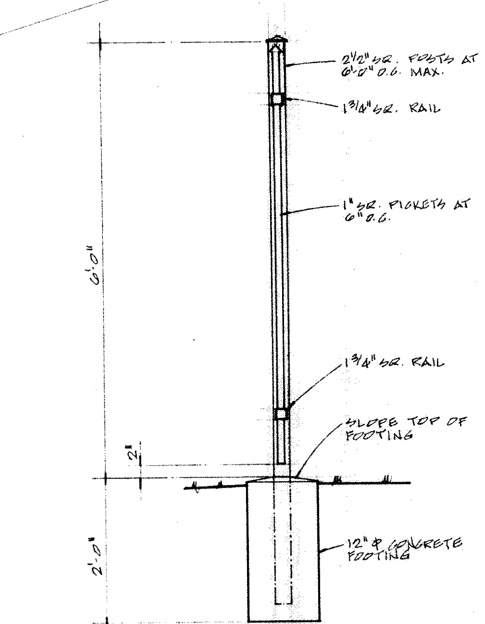
4 SECURITY FENCE
