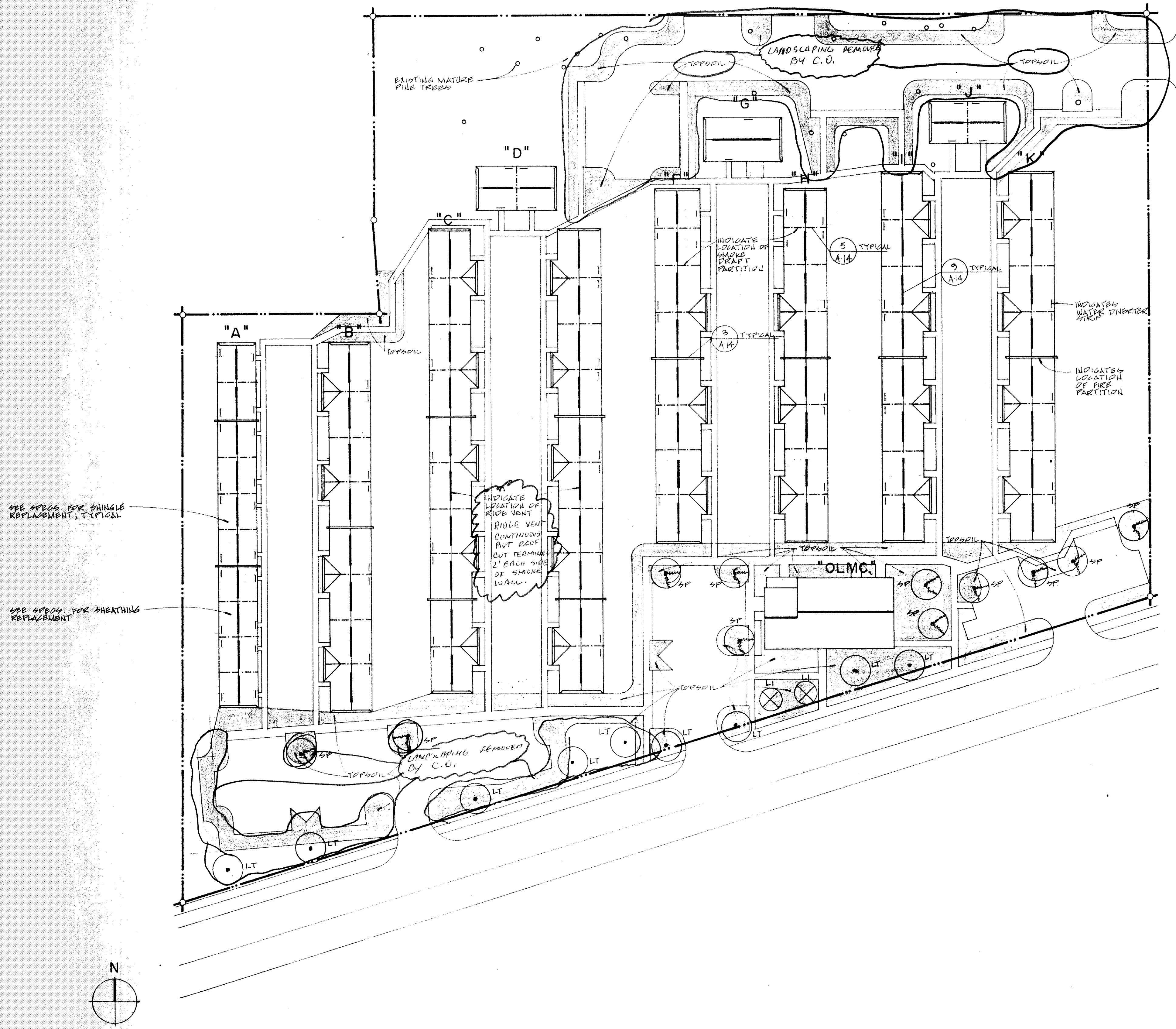
1. ROOF PLAN / LANDSCAPE PLAN
