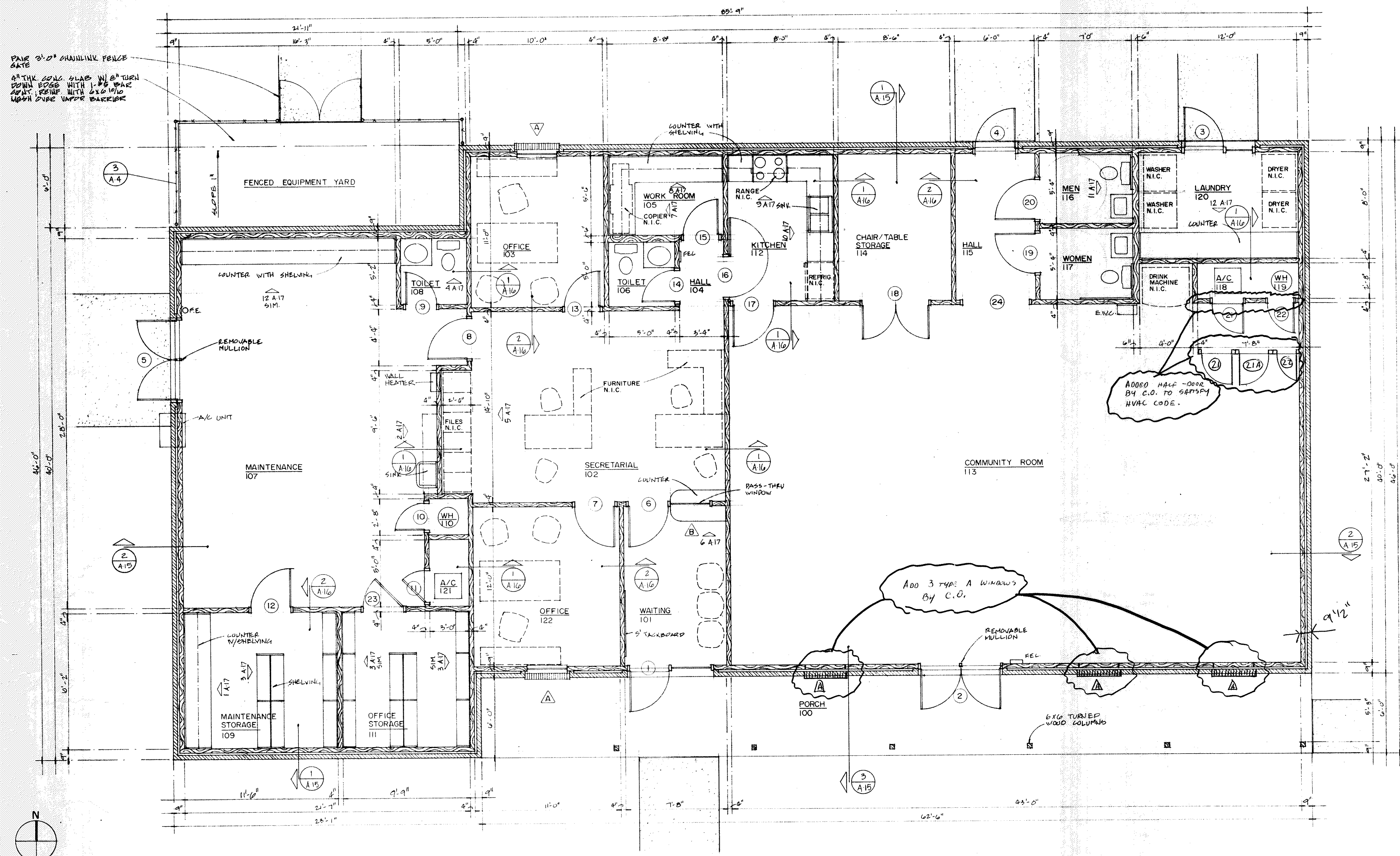
1 A-4 FLOOR PLAN - OFFICE/LAUNDRY/MAINTENANCE/COMMUNITY BUILDING
