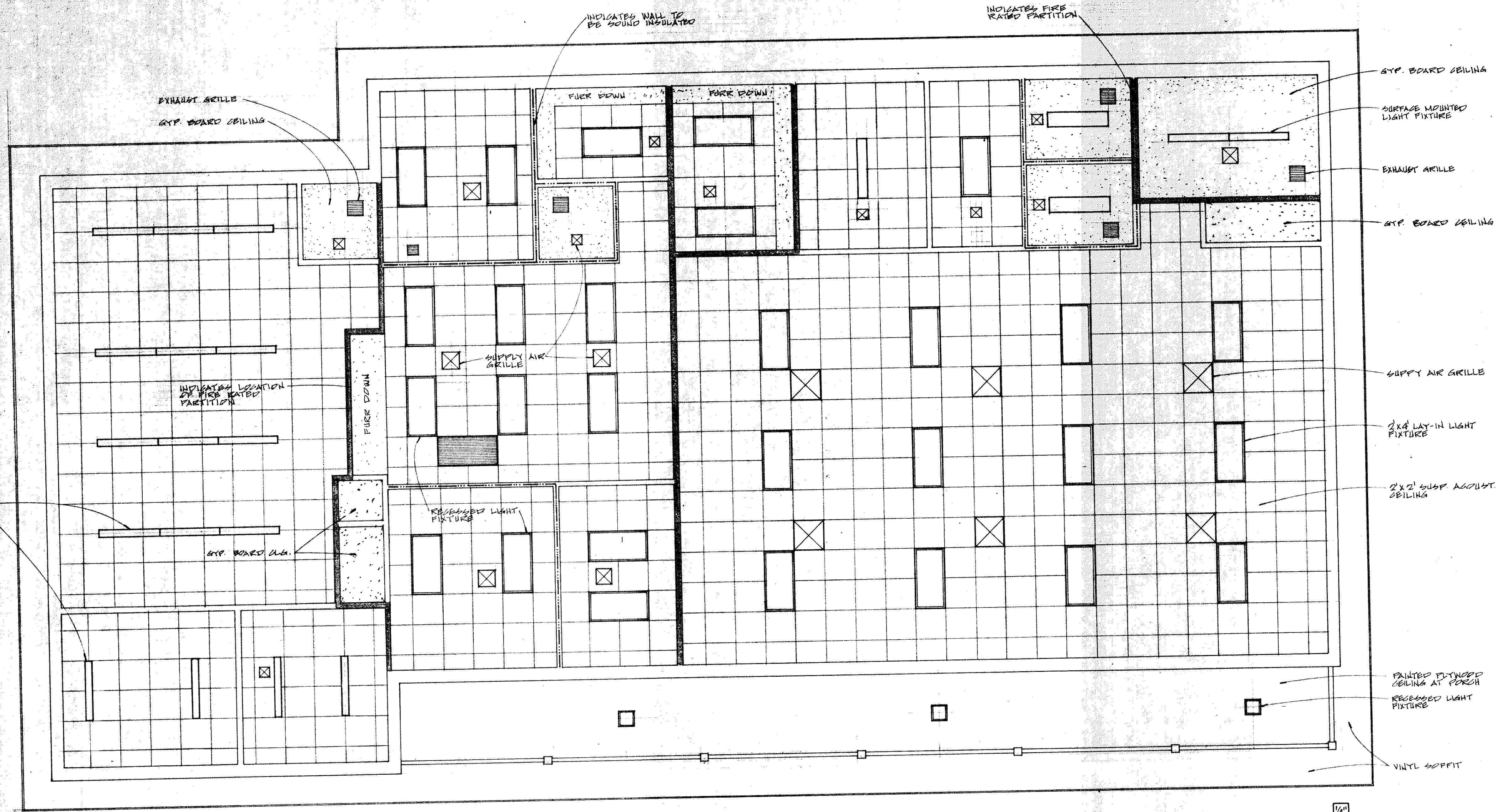
REFLECTED CEILING PLAN - OLMC BUILDING
