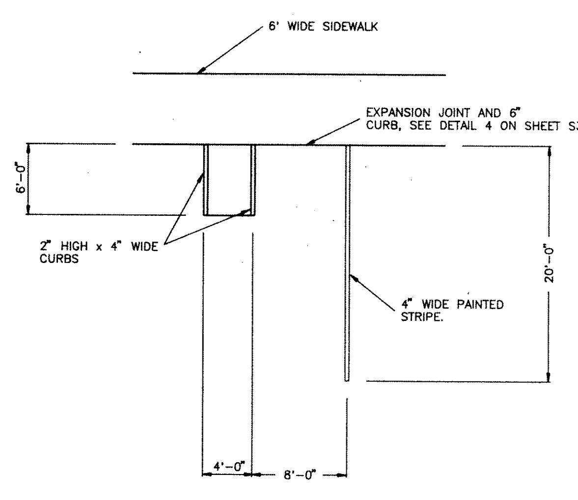
2 HANDICAP PARKING SPACE SCALE 1/8" = 1'-0"
