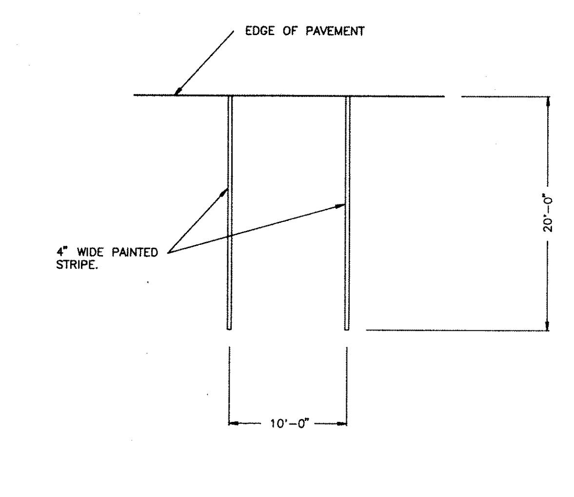
1 TYPICAL PARKING SPACE SCALE 1/8" = 1'-0"
