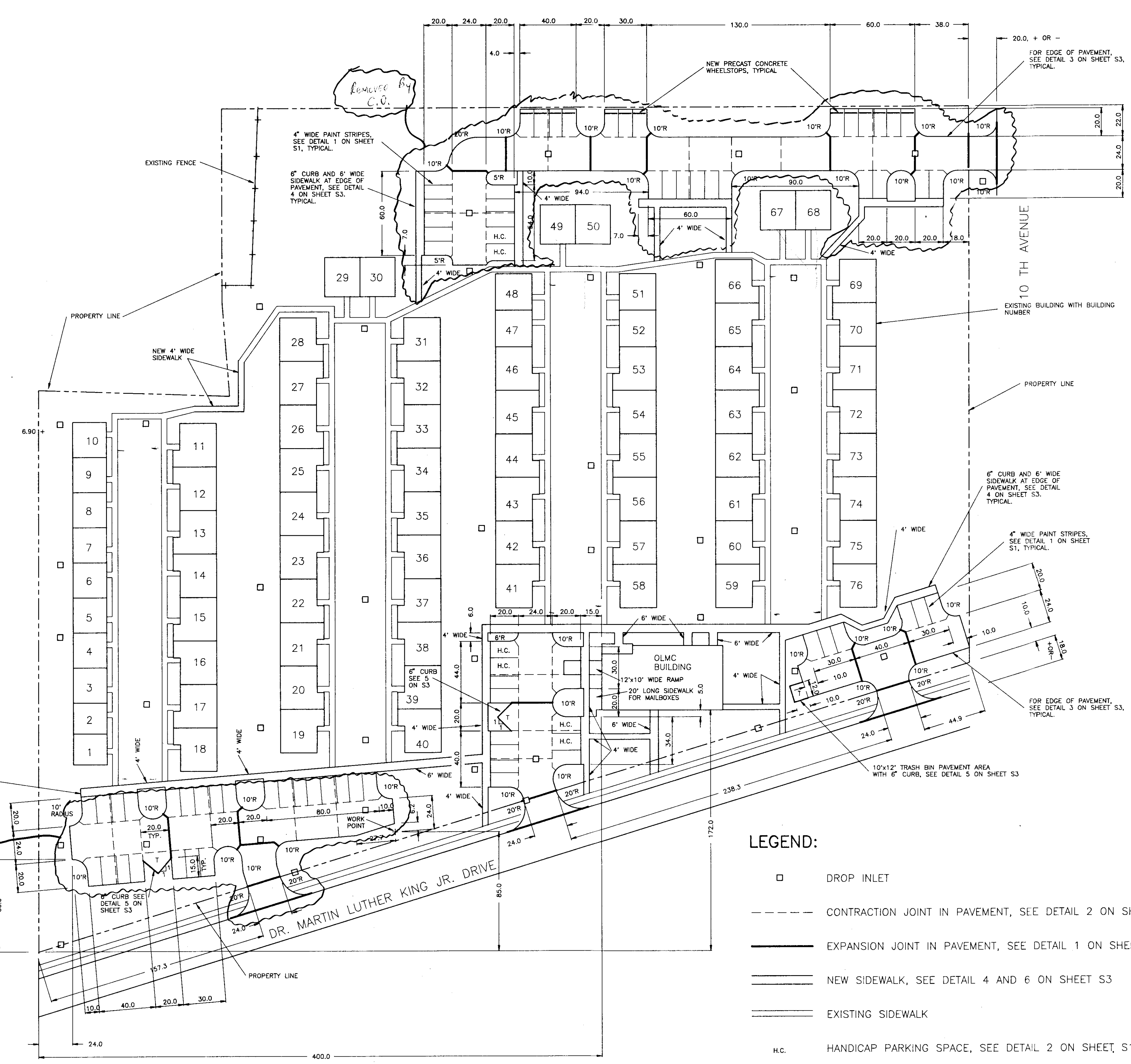
PAVING PLAN SCALE 1" = 40'-0"
