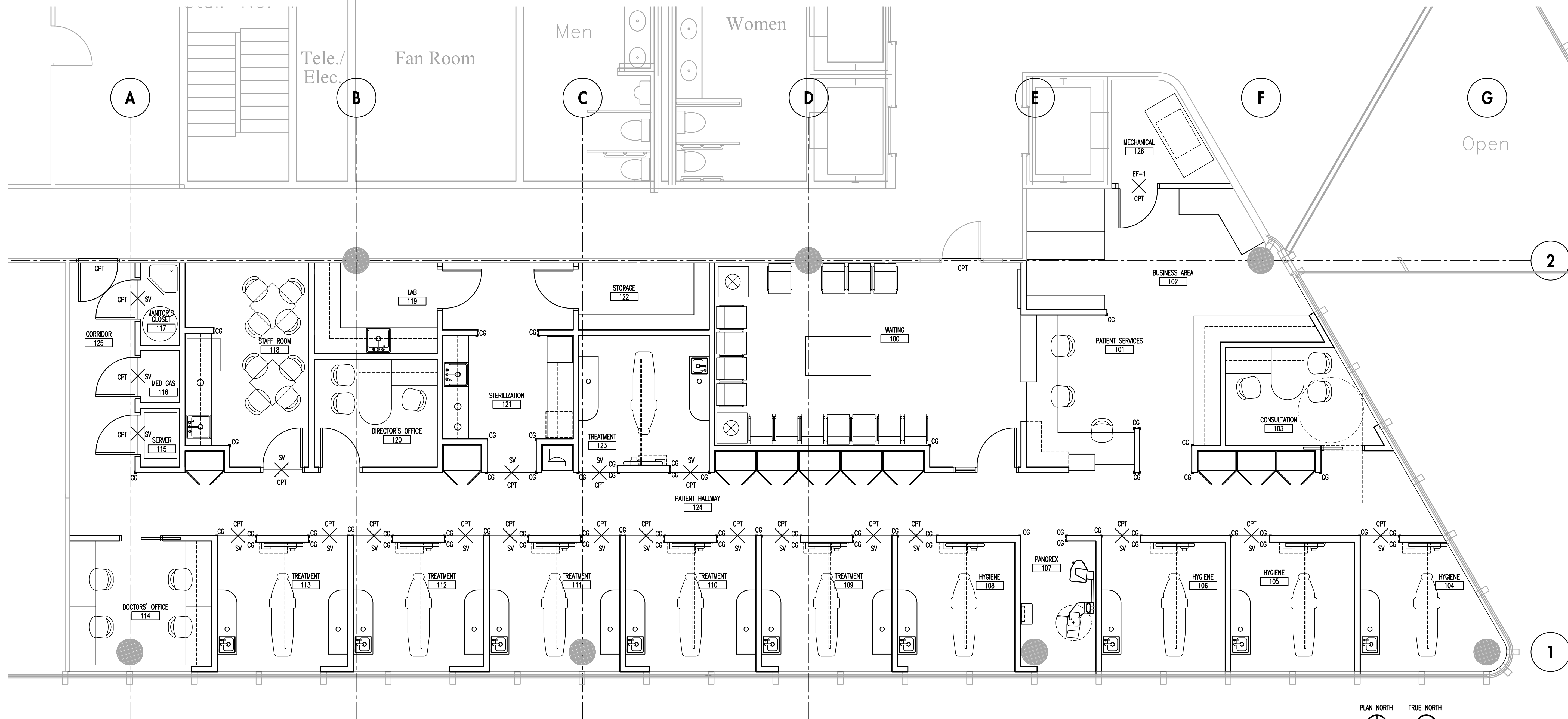
1 Floor Finishes Plan A2.3 SCALE: 1/4"=1'-0"
