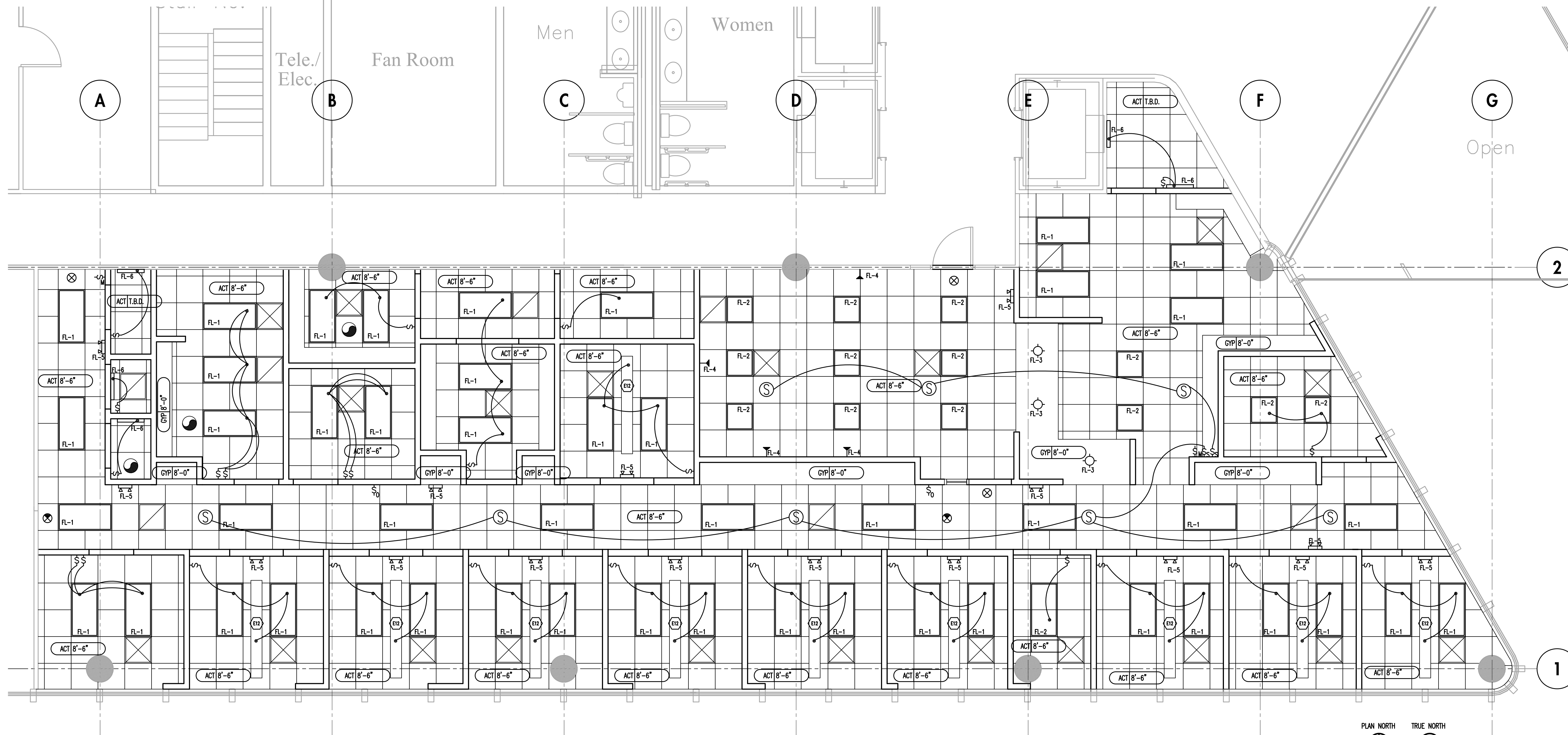
1 Reflected Ceiling Plan SCALE: 1/4"=1'-0"
