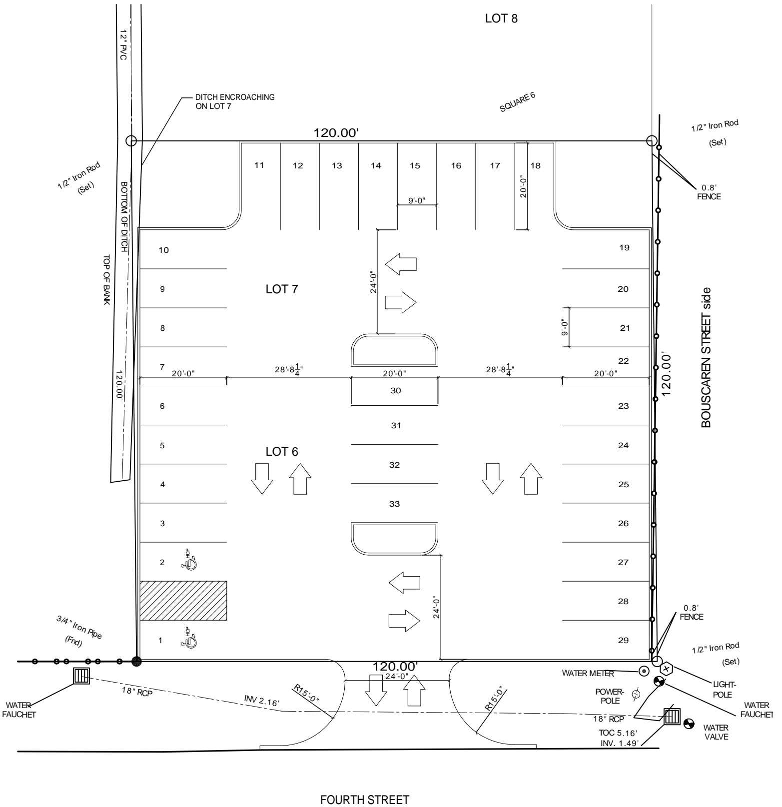
SITE PLAN OPTION "E" SCALE: 1"=10'-0"
