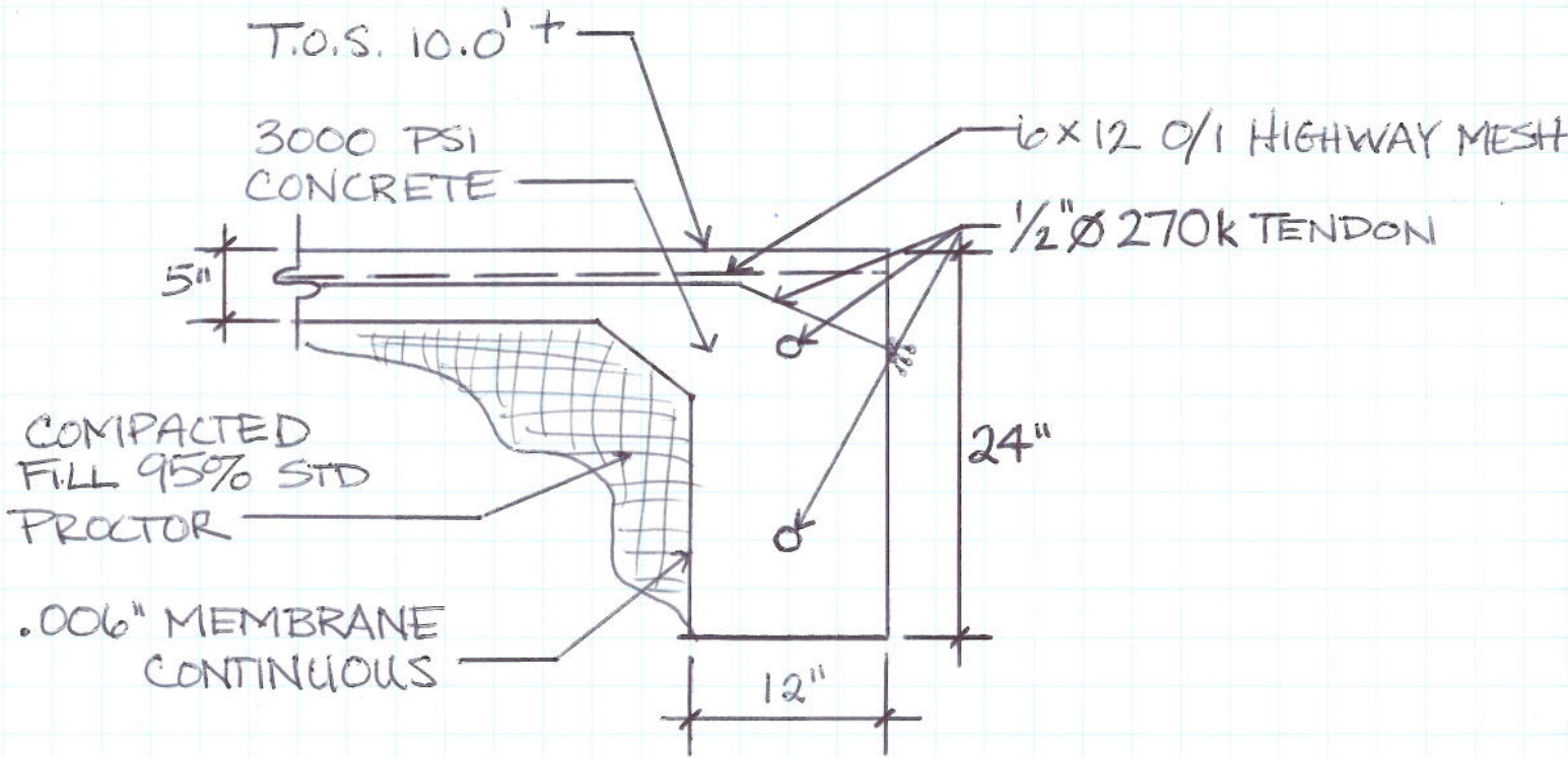
PRELIMINARY FOOTING PLAN
