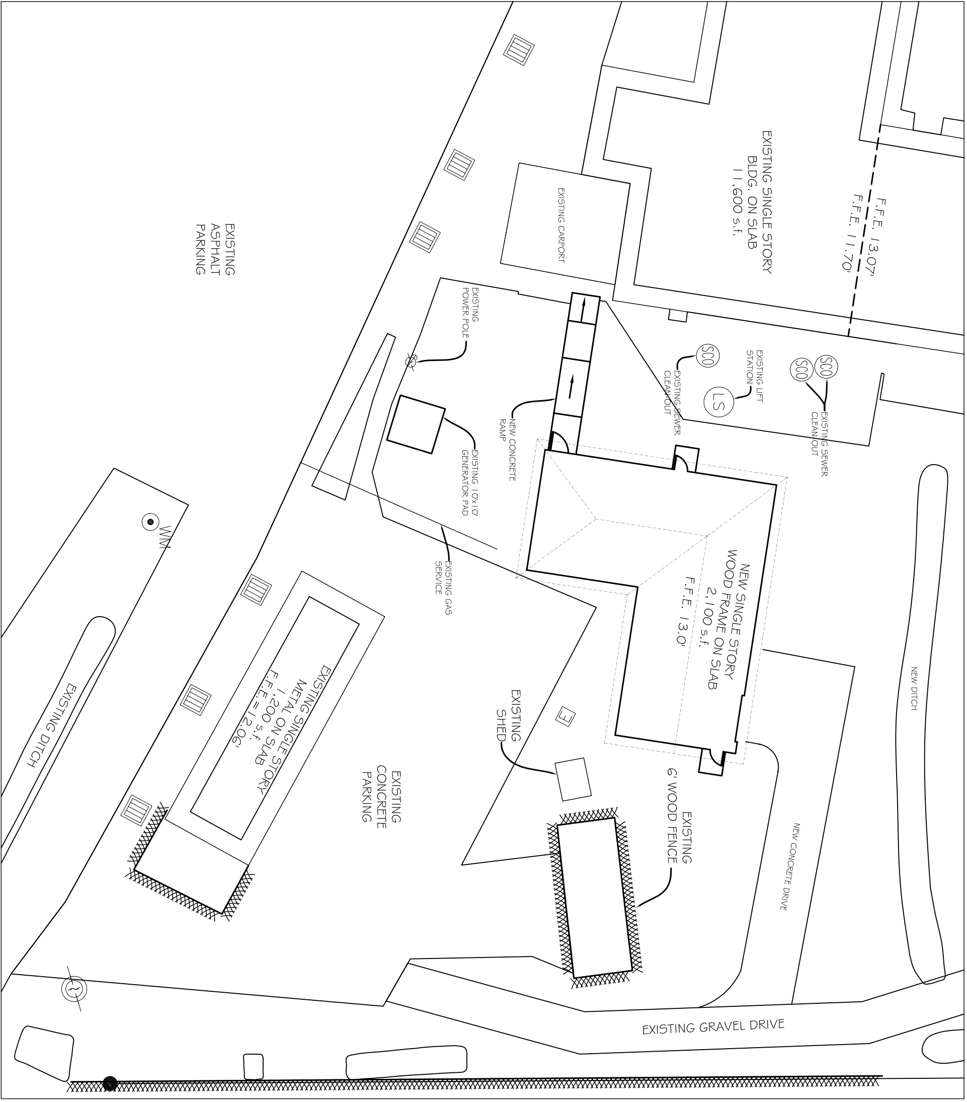
PARTIAL SITE PLAN SCALE: 1" = 10'-0"
