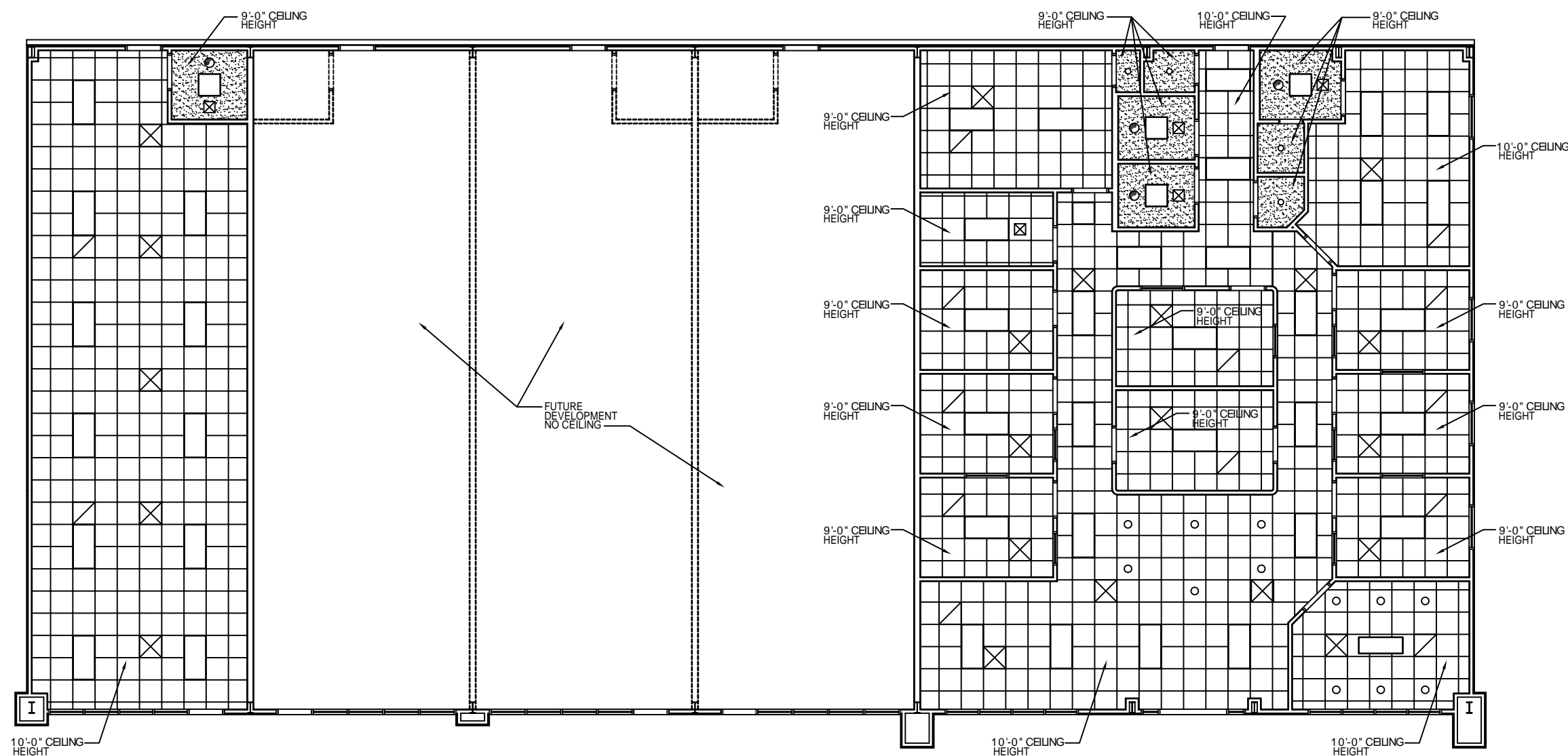
REFLECTED CEILING PLAN SCALE: 3/16"=1'
