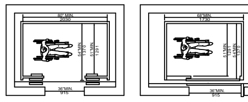
FIG. 22 MINIMUM DIMENSION OF ELEVATOR CARS N.T.S.
