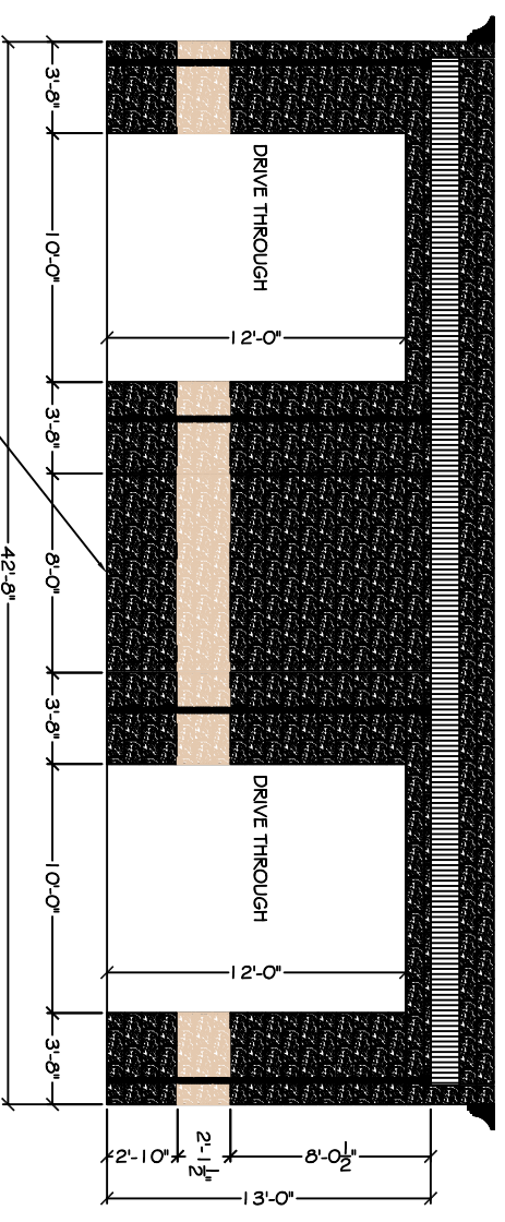
BACK ELEVATION SCALE 1/4" = 1'
