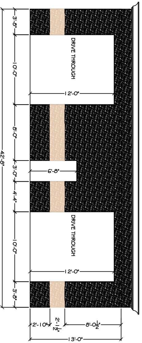
FRONT ELEVATION FACING EAST HALL SCALE 1/4" = 1'
