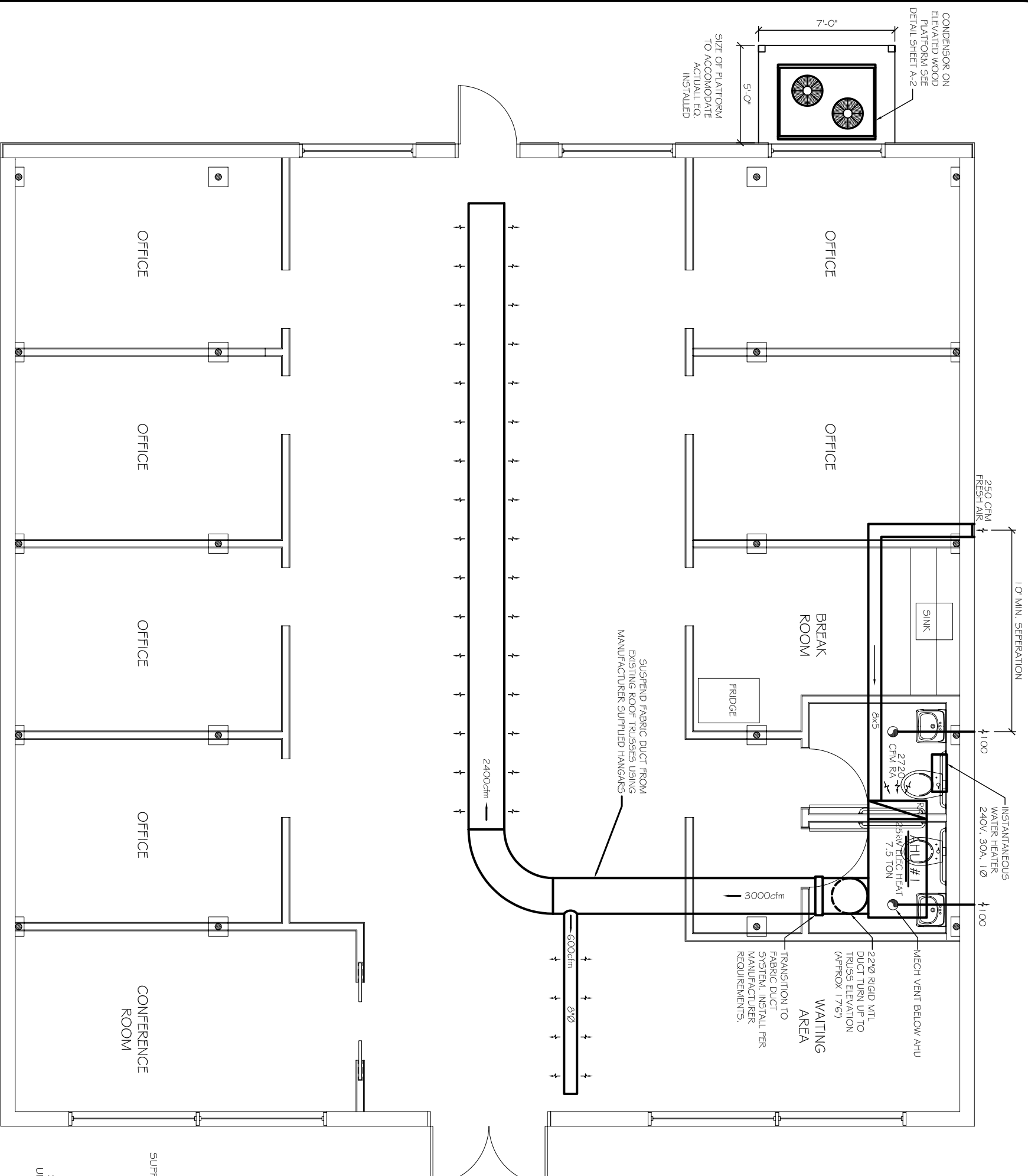
MECHANICAL PLAN SCALE: 3/8" = 1'
