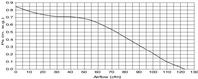
MODEL QTX110SL
