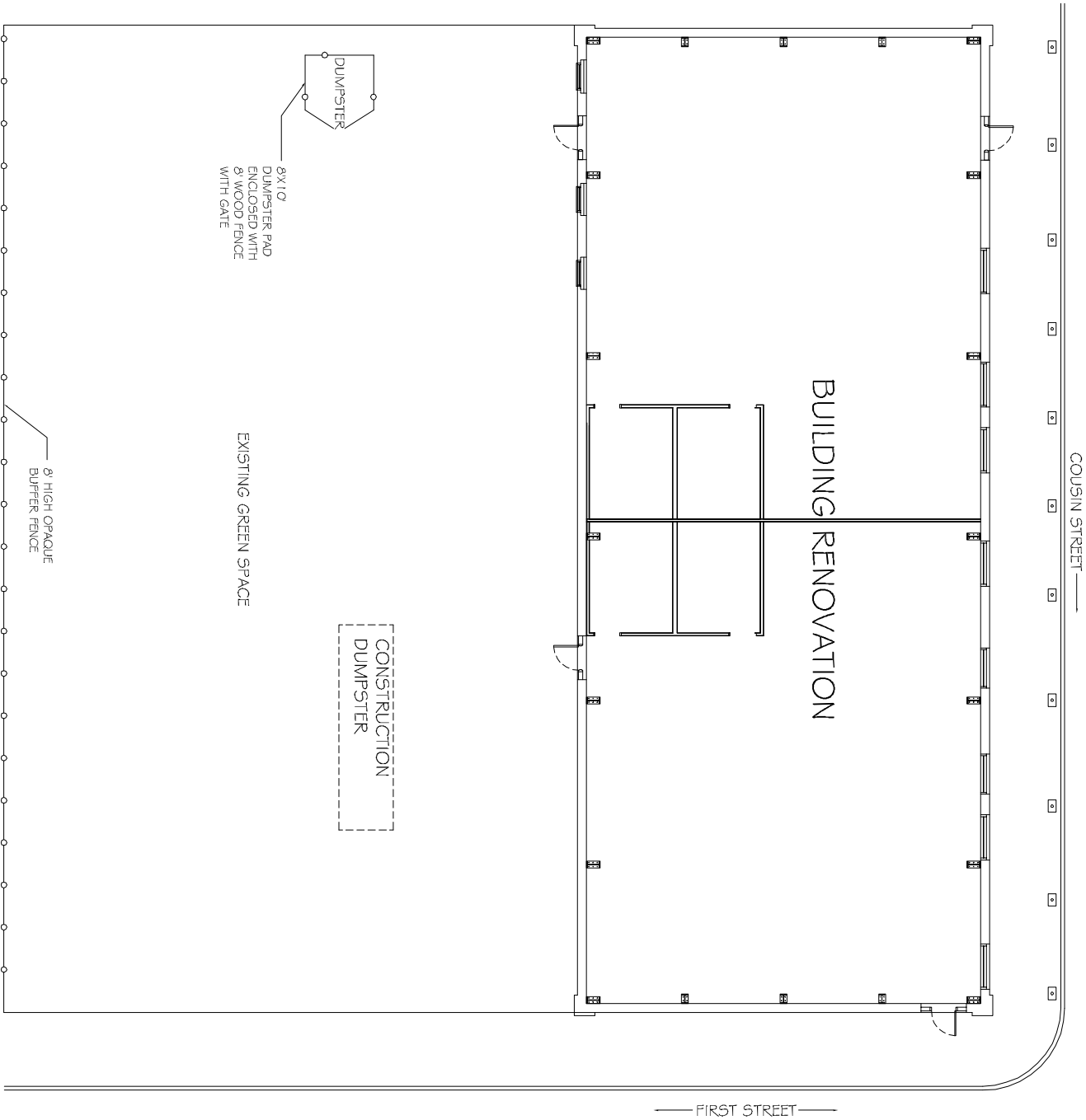
ELECTRICAL SITE PLAN SCALE: 3/32"=1'-0"
