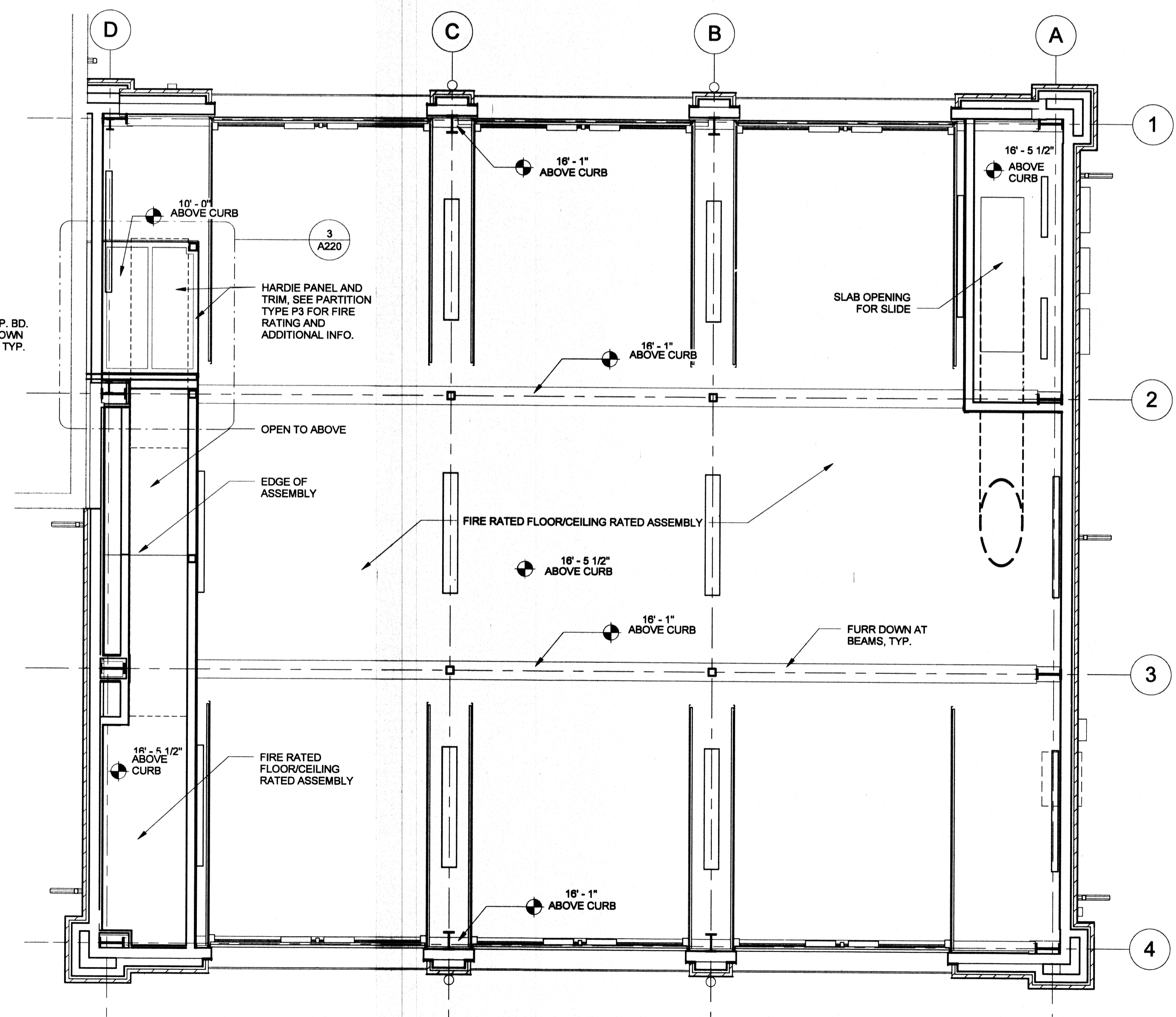
2 First Floor Ceiling Plan A220 3/16" = 1'-0"
