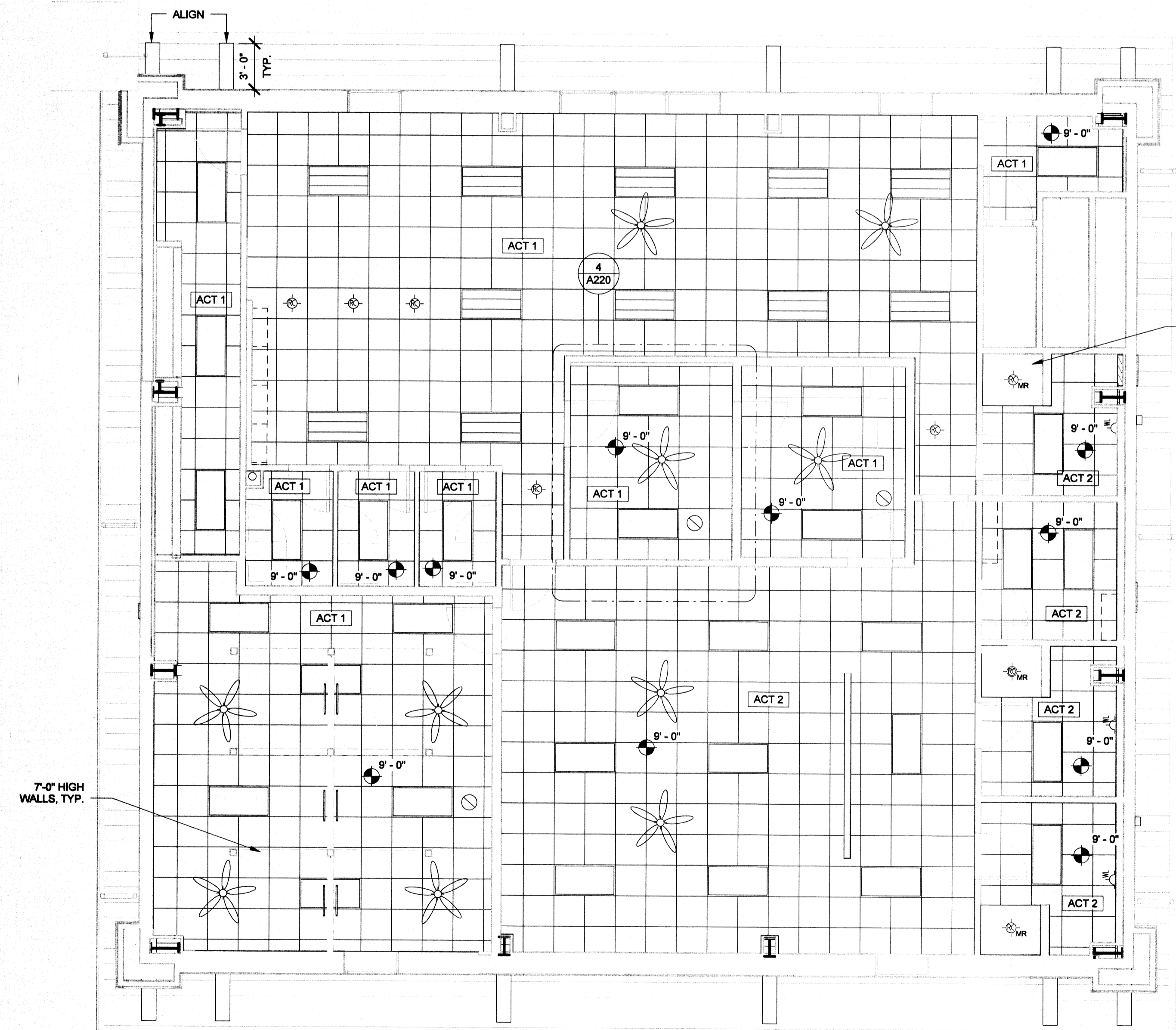
1 Second Floor Ceiling Plan A220 3/16" = 1'-0"
