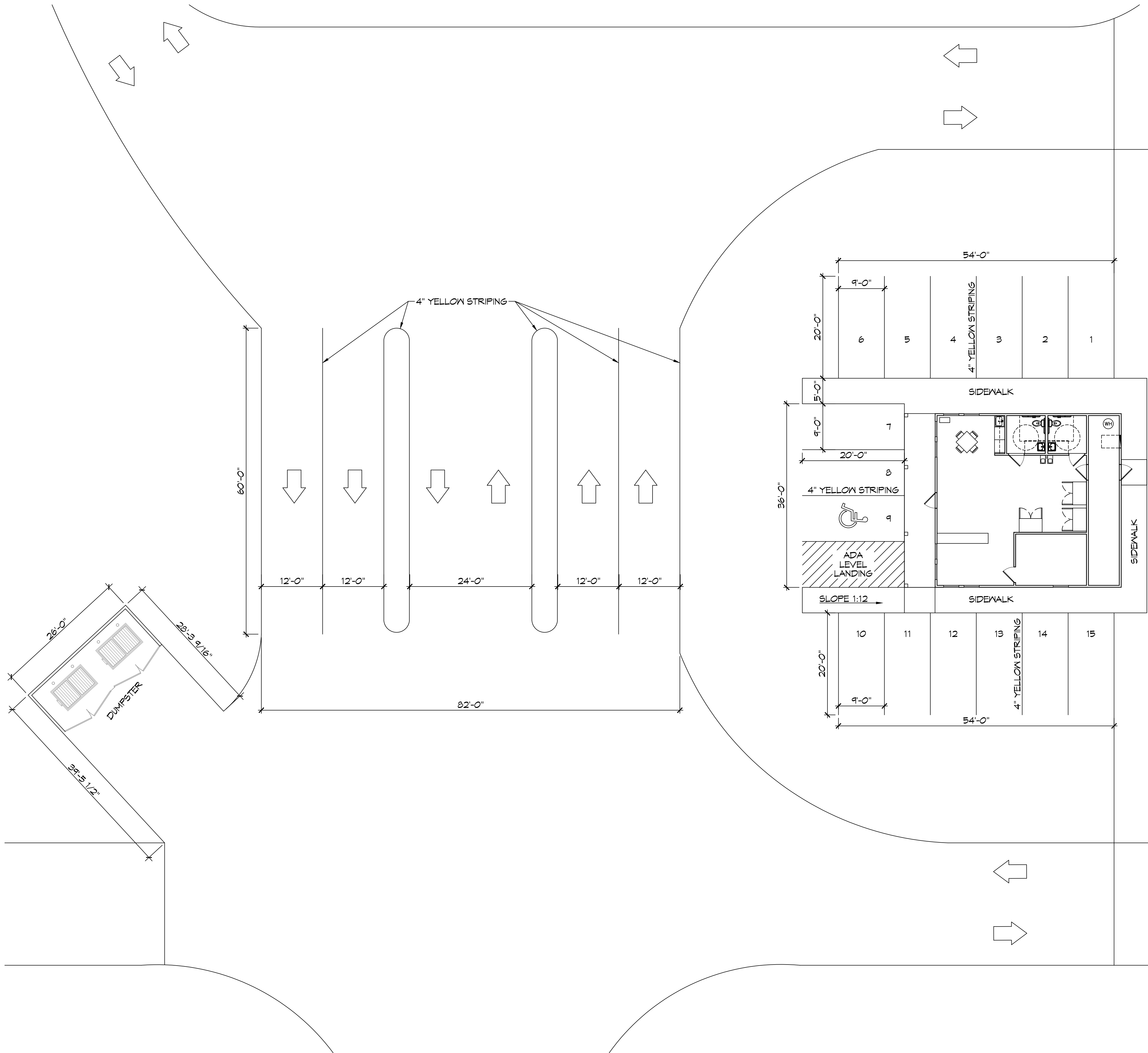
12 WELCOME CENTER PARKING PLAN SCALE: 1" = 10'-0"
